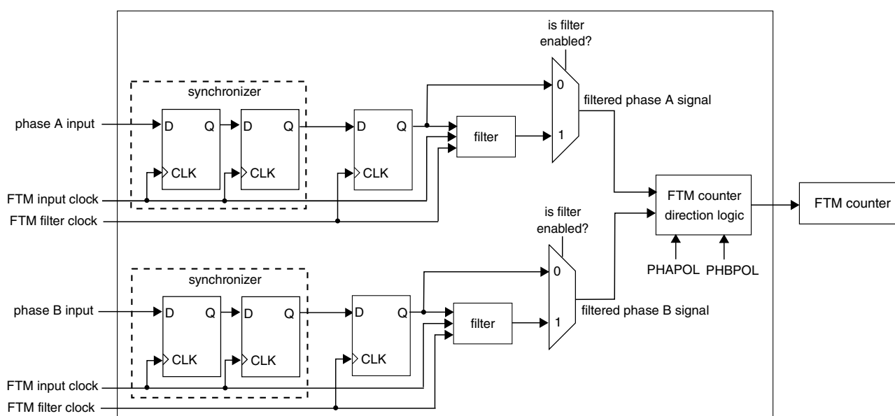
Figure 41-102. Diagram for Quadrature Decoder when FLTPS[3:0] \neq 0
