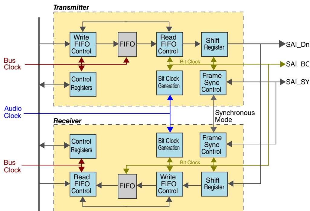
Figure 50-1. MCXE247 SAI Block Diagram
