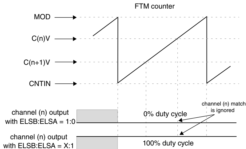
Figure 41-40. Channel (n) output if (\text{CNTIN} < C(n)V < \text{MOD}) and (\text{CNTIN} < C(n+1)V < \text{MOD}) and C(n)V > C(n+1)V
