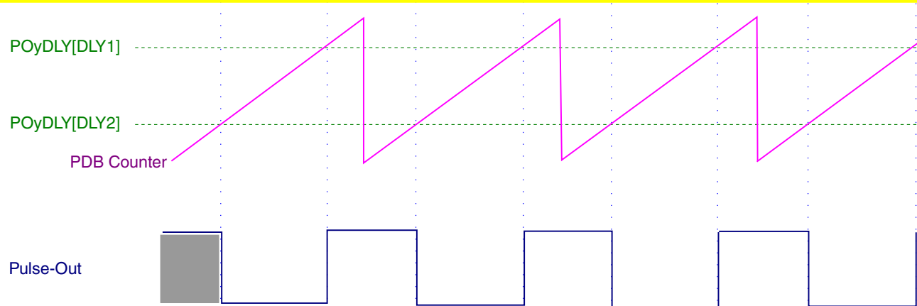
Figure 40-9. How Pulse Out is generated
