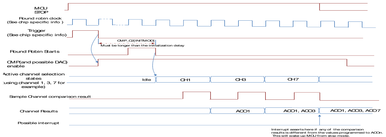
Figure 39-16. Trigger mode
