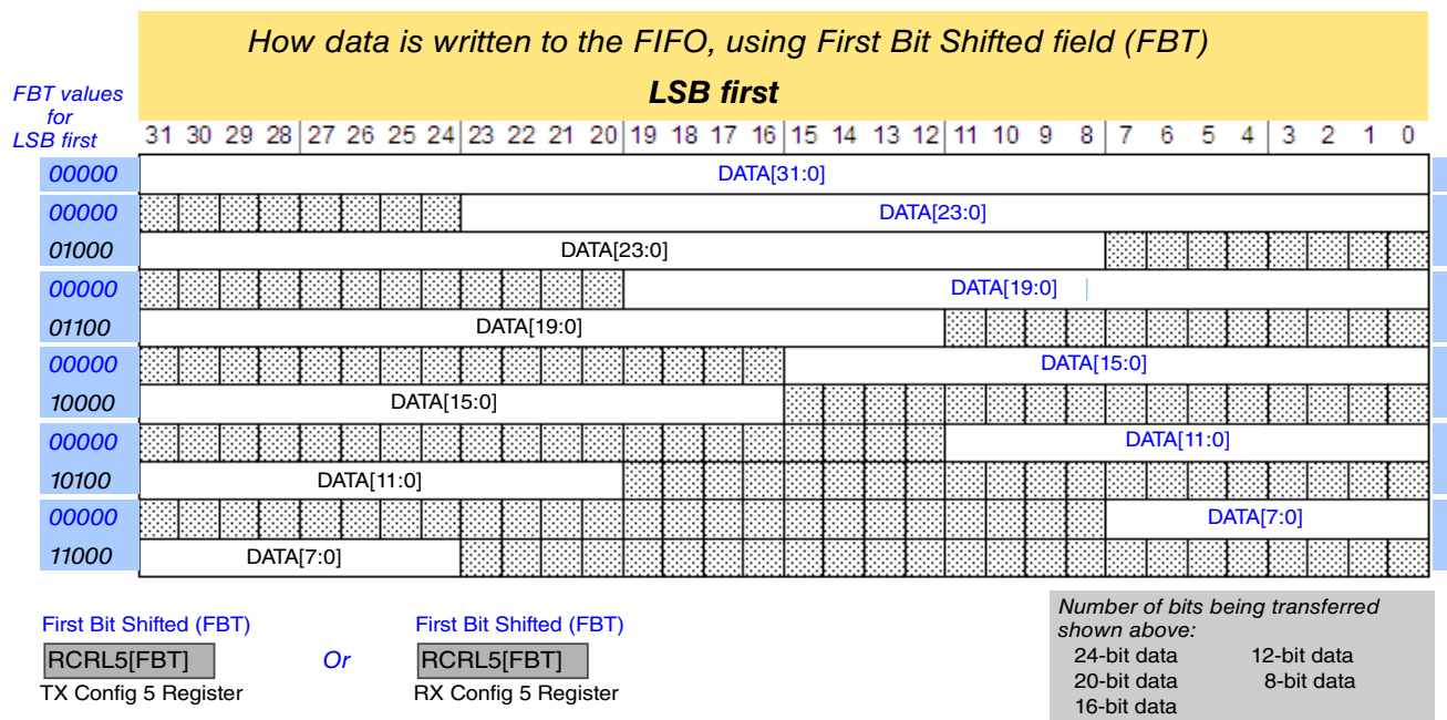
Figure 50-3. SAI first bit shifted, LSB first
