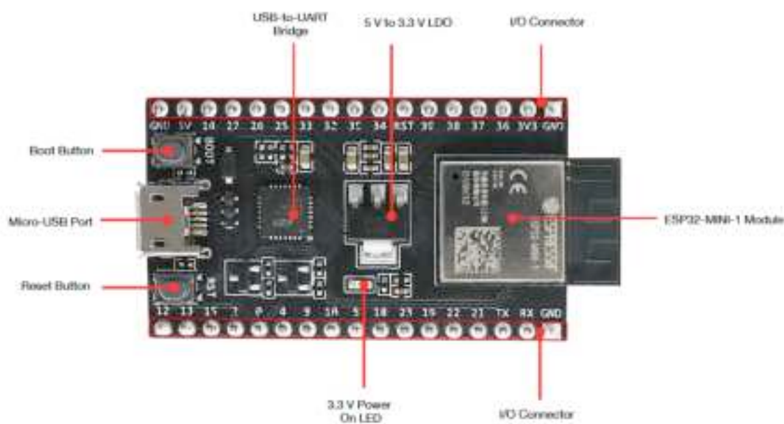
Fig. 6: ESP32-DevKitM-1 - front
