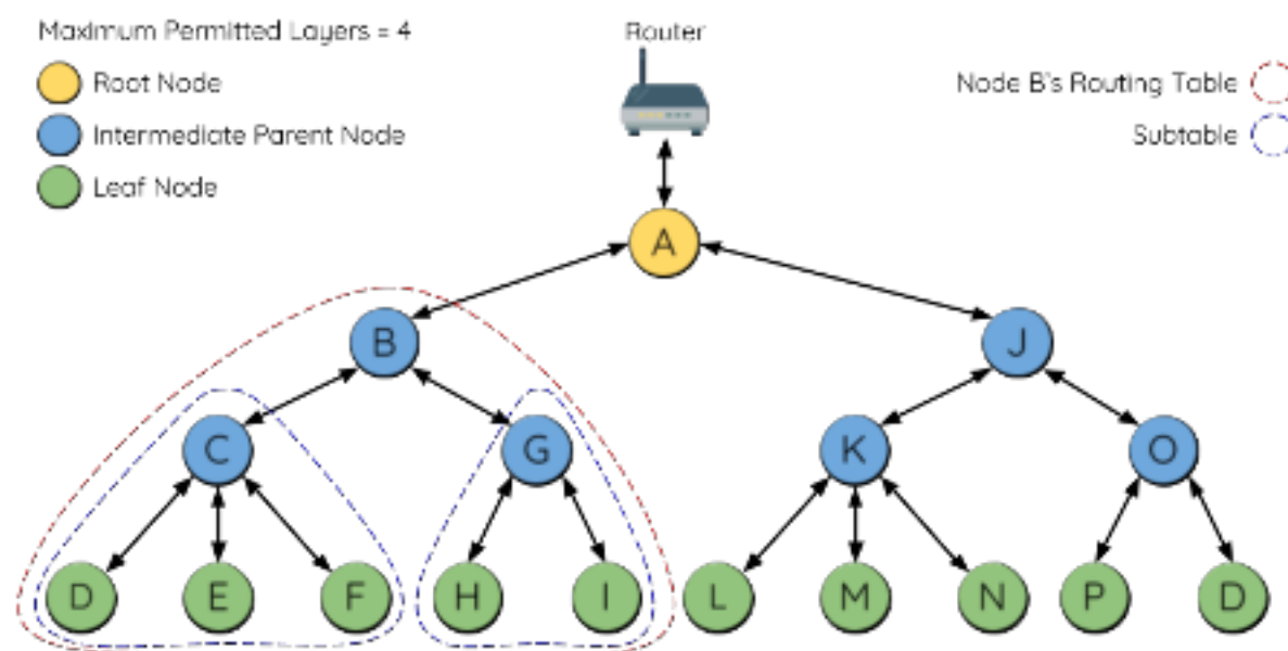
Fig. 47: ESP-WIFI-MESH Routing Tables Example
