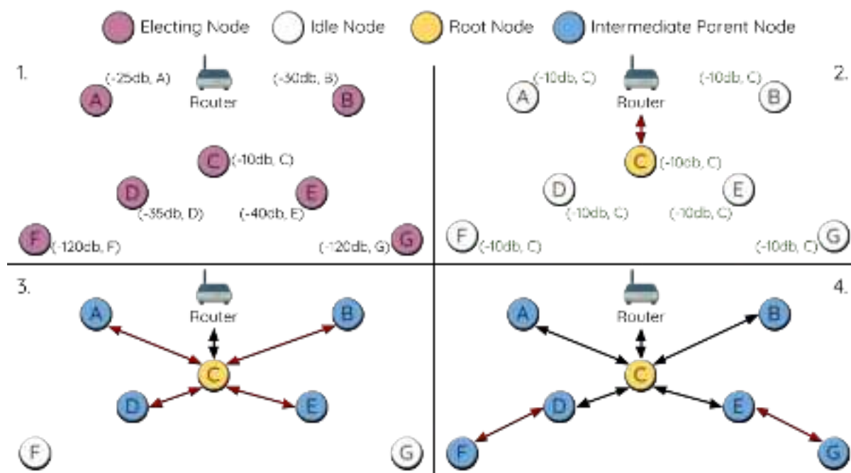
Fig. 49: Root Node Election Example
