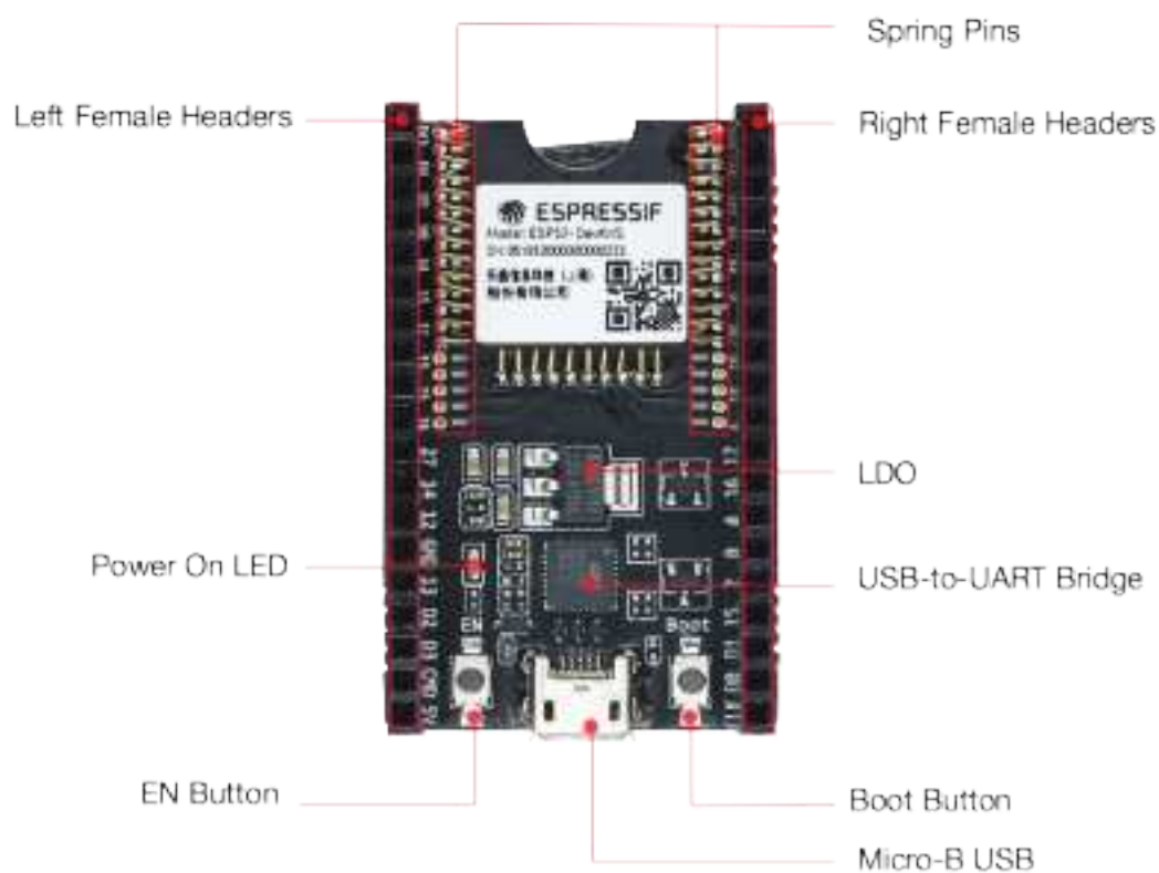
Fig. 1: ESP32-DevKitS - front
