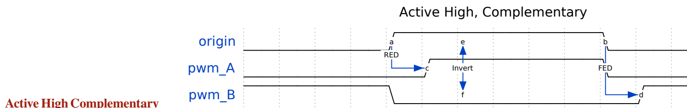
Active High Complementary
