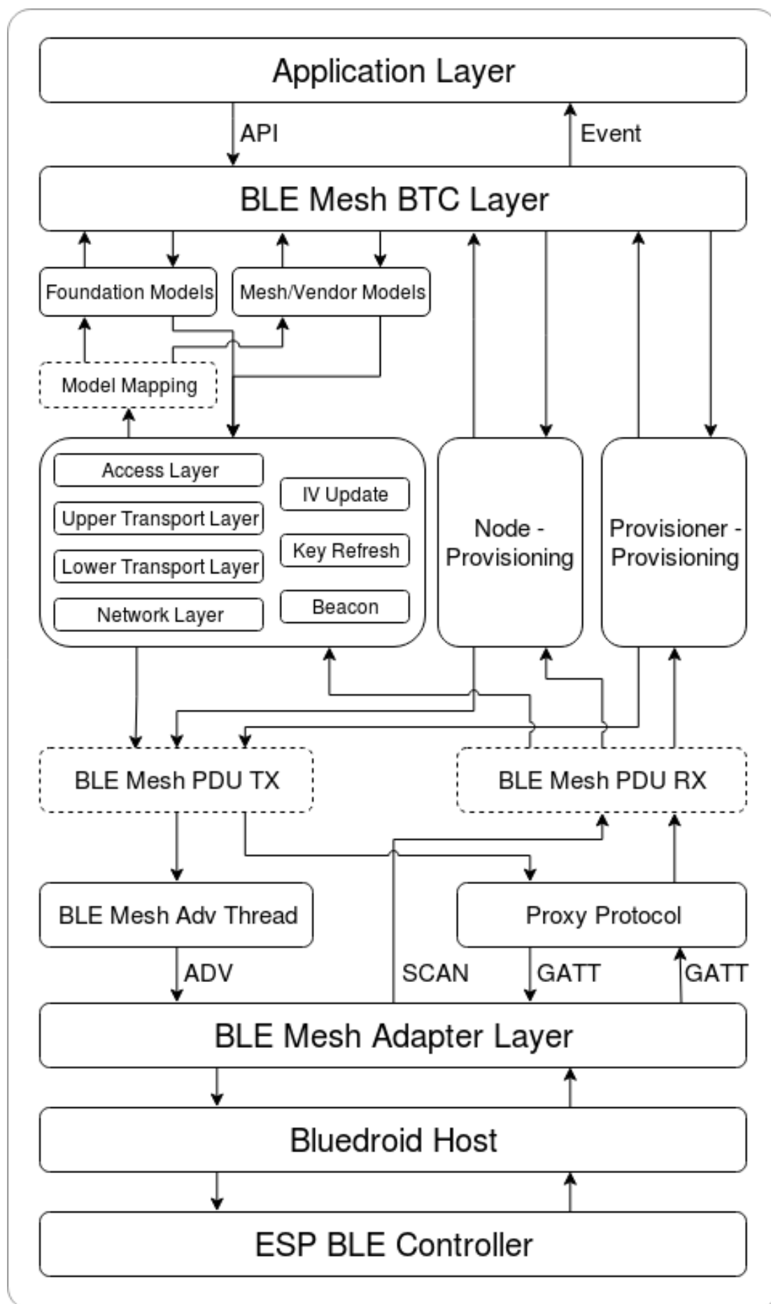
Fig. 35: Figure 2.1 ESP-BLE-MESH Architecture Implementation Diagram
