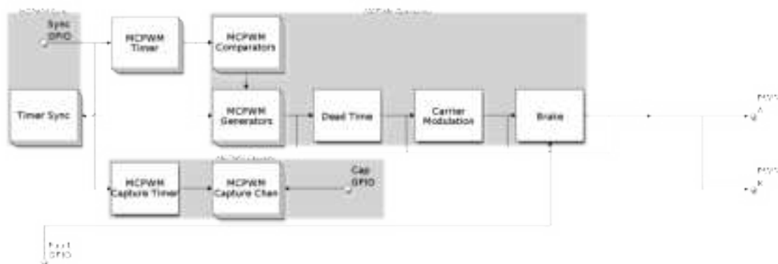
Fig. 12: MCPWM Overview
