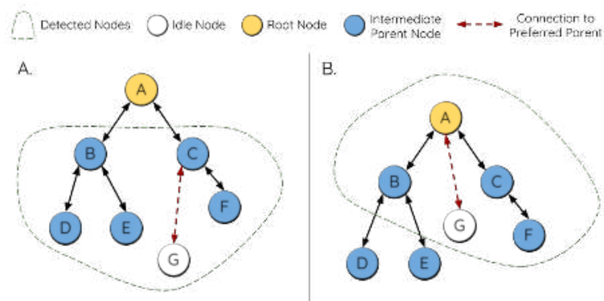
Fig. 46: Preferred Parent Node Selection
