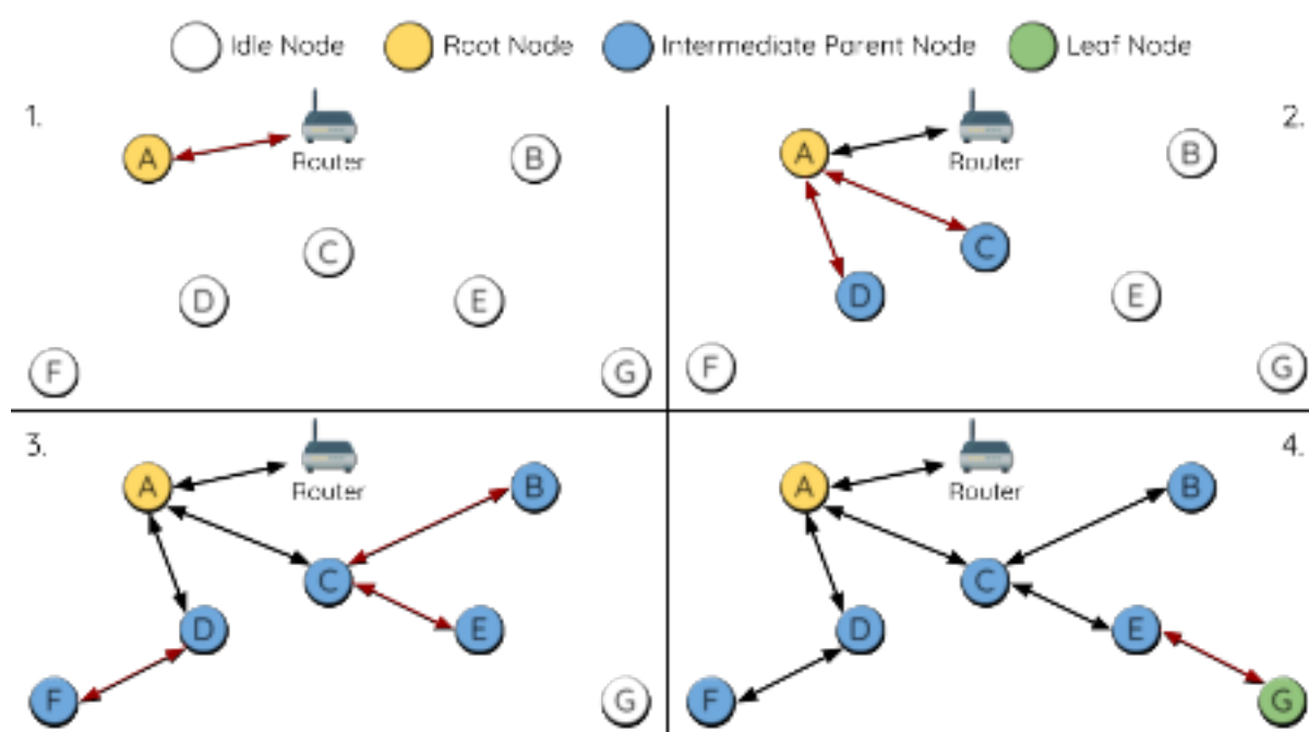
Fig. 50: Root Node Designation Example (Root Node = A, Max Layers = 4)
