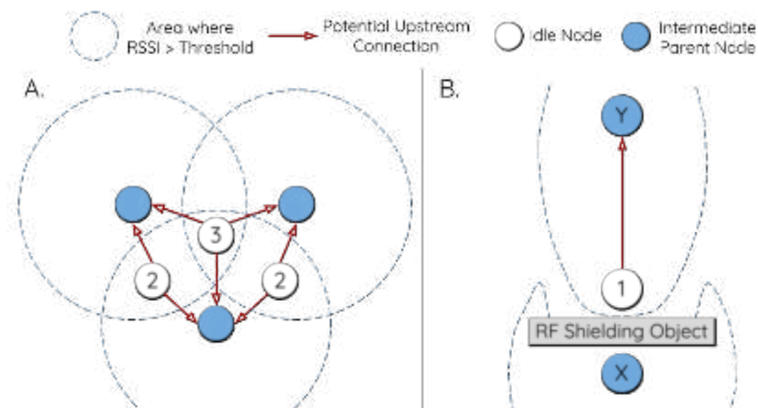
Fig. 45: Effects of RSSI Thresholding
