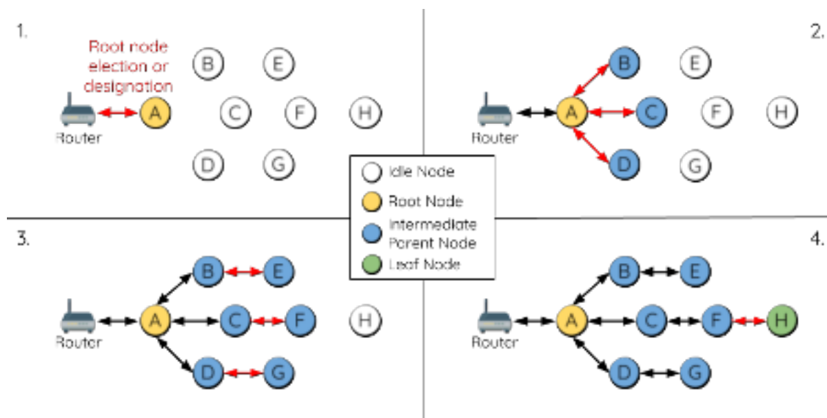
Fig. 48: ESP-WIFI-MESH Network Building Process
