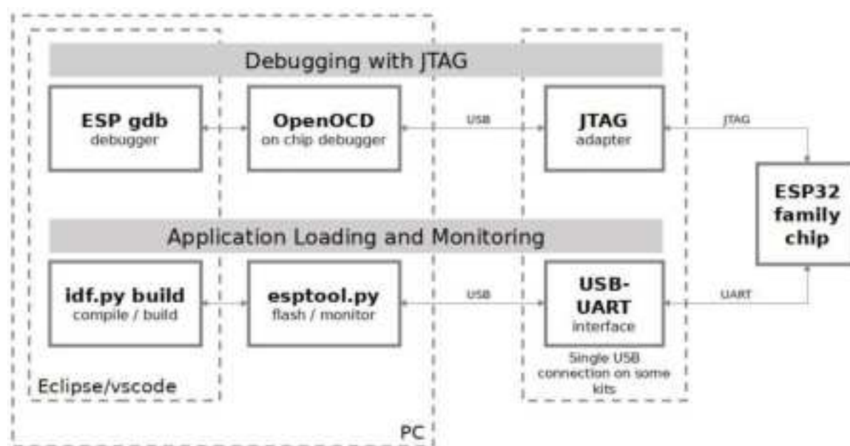
Fig. 58: JTAG debugging - overview diagram
