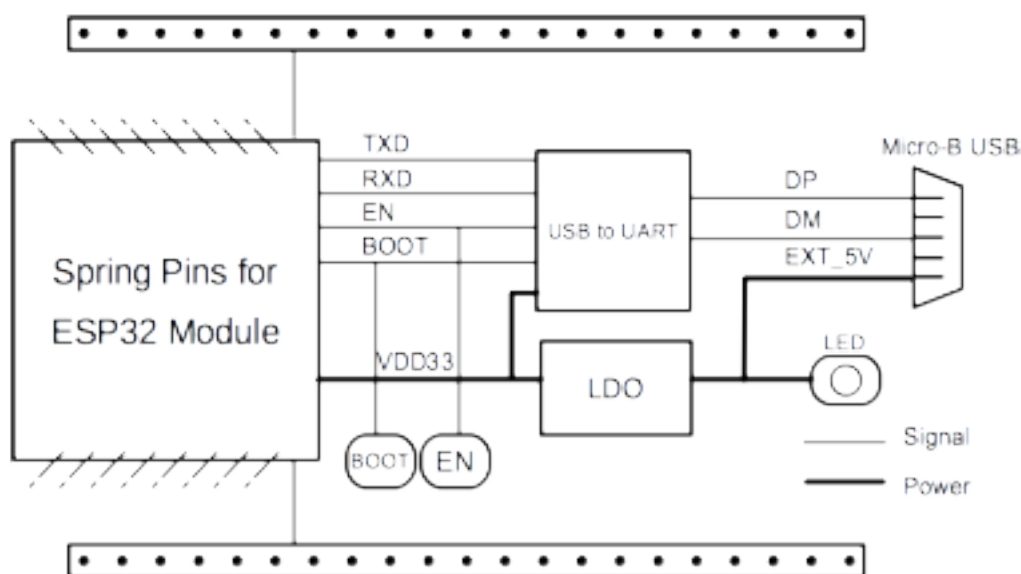
Fig. 5: ESP32-DevKitS(-R) (click to enlarge)
