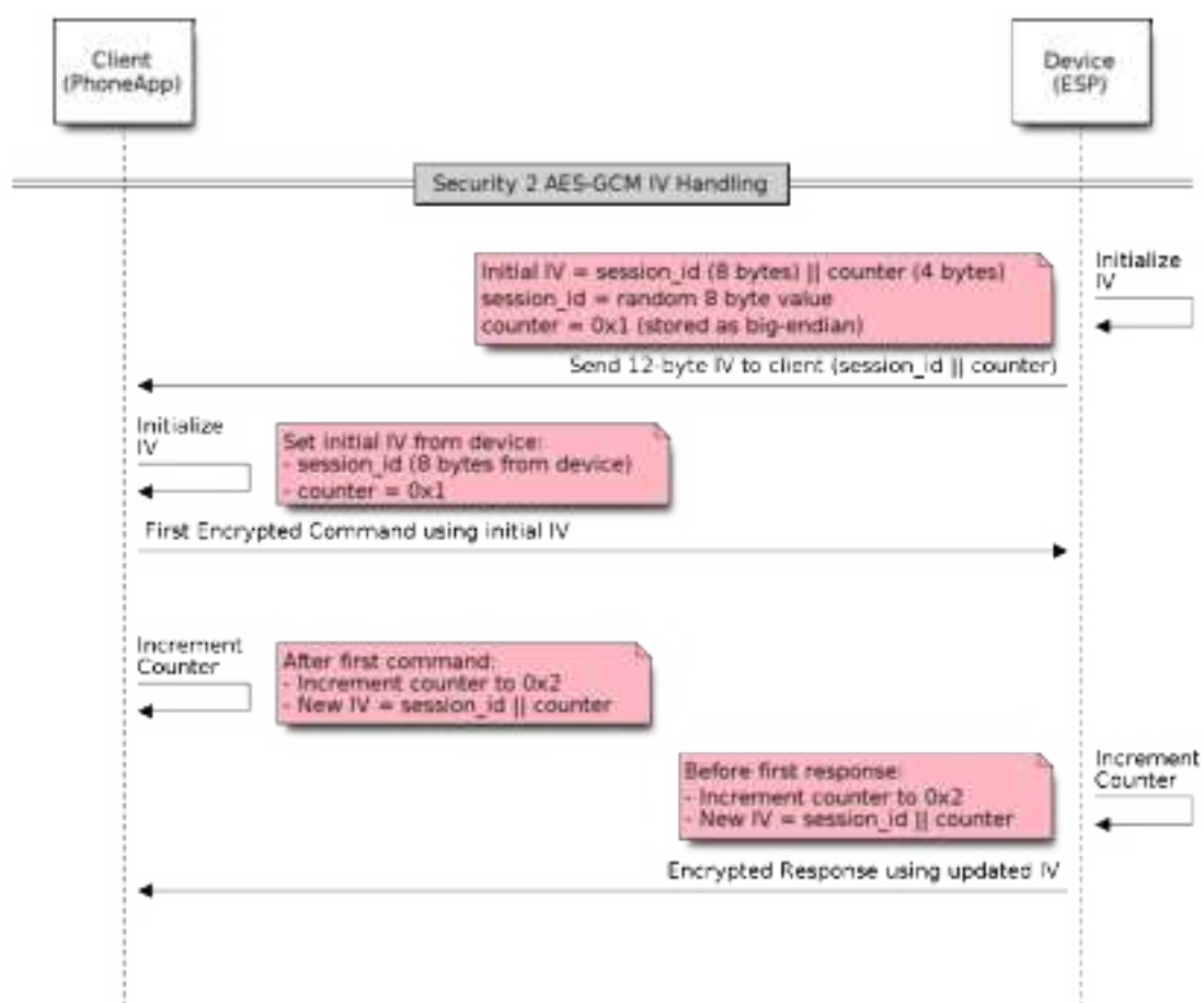
Fig. 32: Security 2 AES-GCM IV Handling
