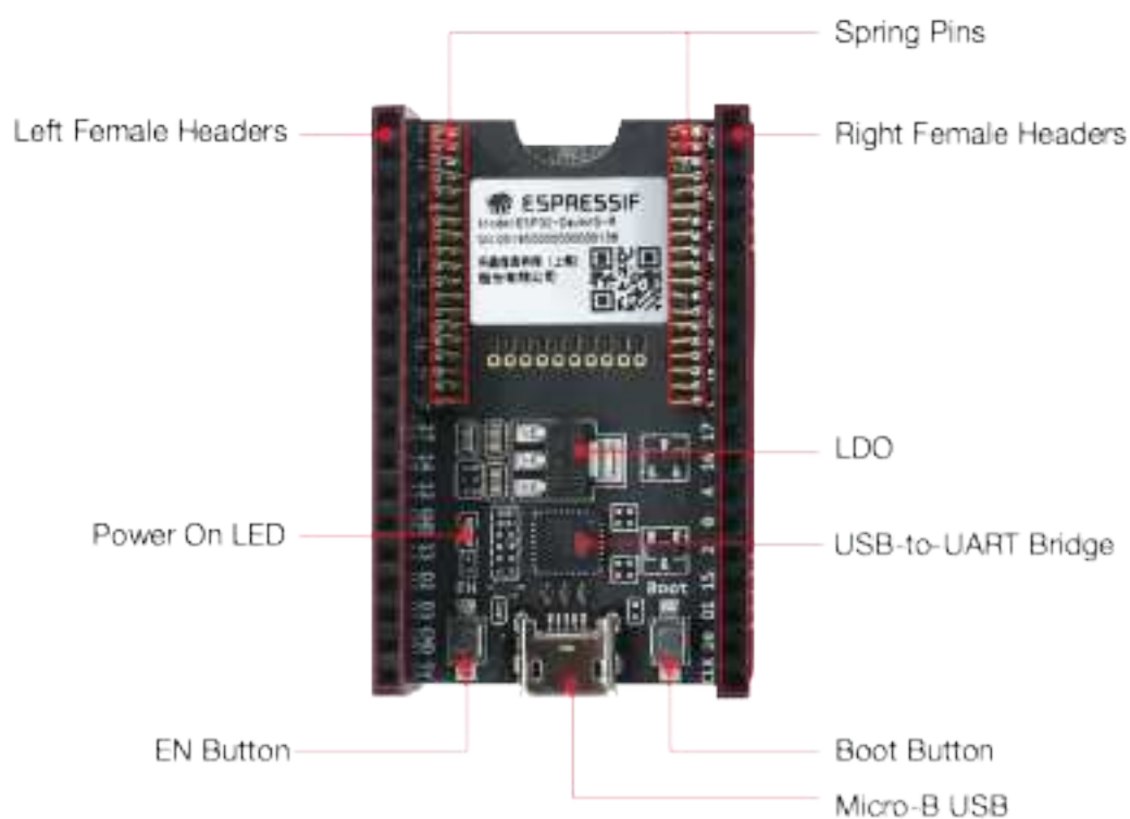
Fig. 2: ESP32-DevKitS-R - front
