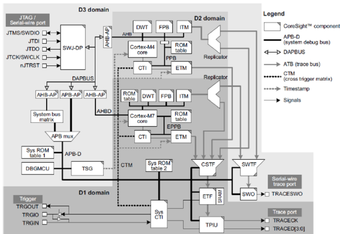
Figure 20. Block diagram of the device debug
