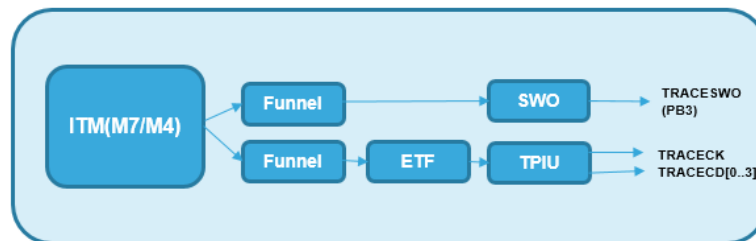
Figure 22. Block diagram of ITM debug
