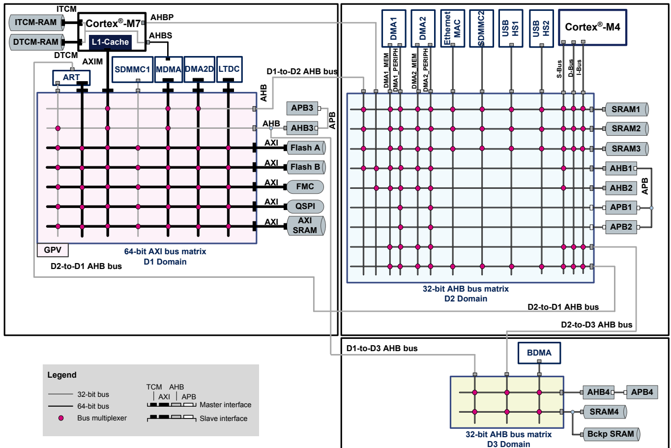
Figure 2. STM32H7 dual-core system architecture
