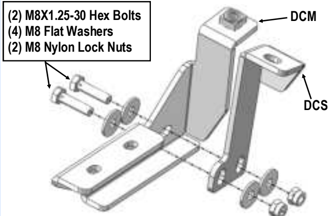
(Fig 10) Driver Side Center Bracket Assembly
