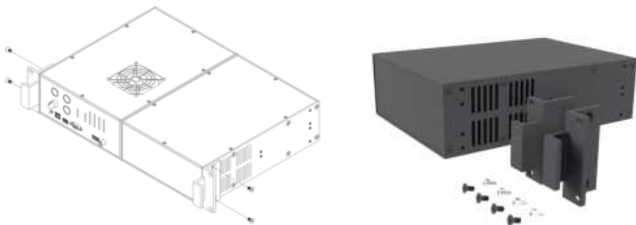
Figure 11. Single rack kit (SingleRackKit-2U)
