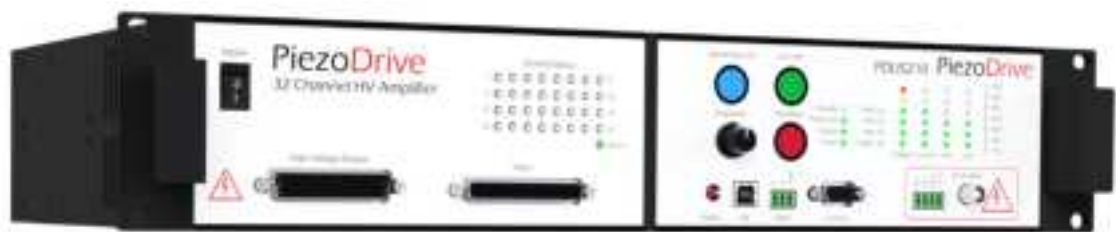
Figure 12. Example double rack option with a PDUS210 (right) and PD32 (left).
