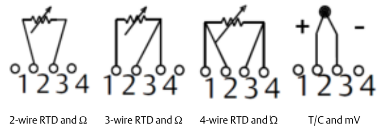
Figure 5-2: Sensor Connections
