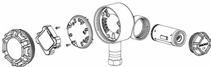
Figure 3-1: Exploded View of LCD Display Assembly
