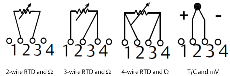
Figure 5-2: Sensor Connections
