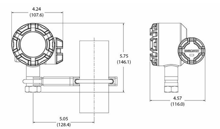
Figure 3-4: Remote Mount
