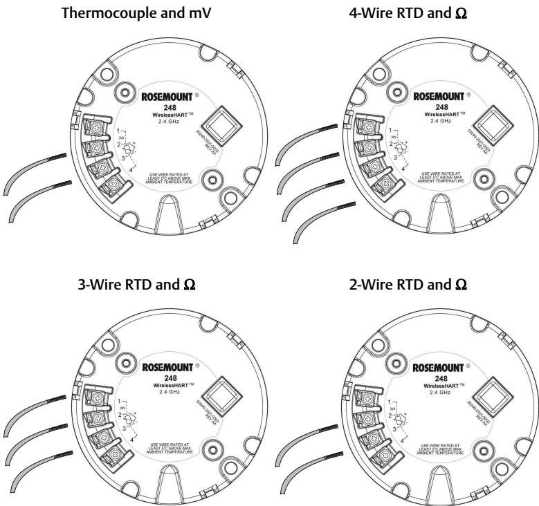
Figure 5-1: Sensor Wiring
