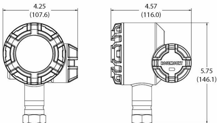
Figure 3-2: Direct Mount
