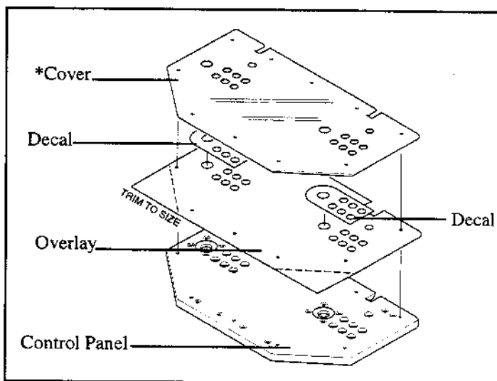
Figure 1 Overlay Installation
