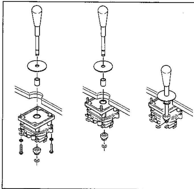
FIGURE 4 Joystick Installation
