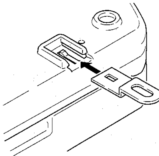
Figure 10: Mounting Bracket Installation
