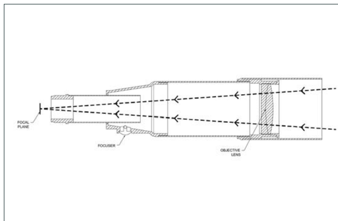
Figure 3-1 A cutaway view of the light path of the Refractor optical design
