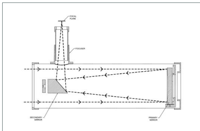
Figure 3-1 Cutaway view of the light path of the Newtonian
