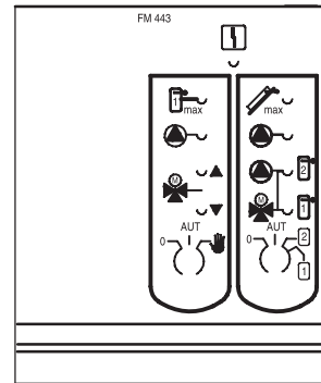
Module – front view
