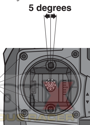
Set screws
