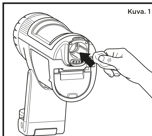
DIRTDETECT-LIANTUNNISTUSANTURI
