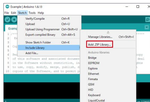
Figure 3. Software Installation
