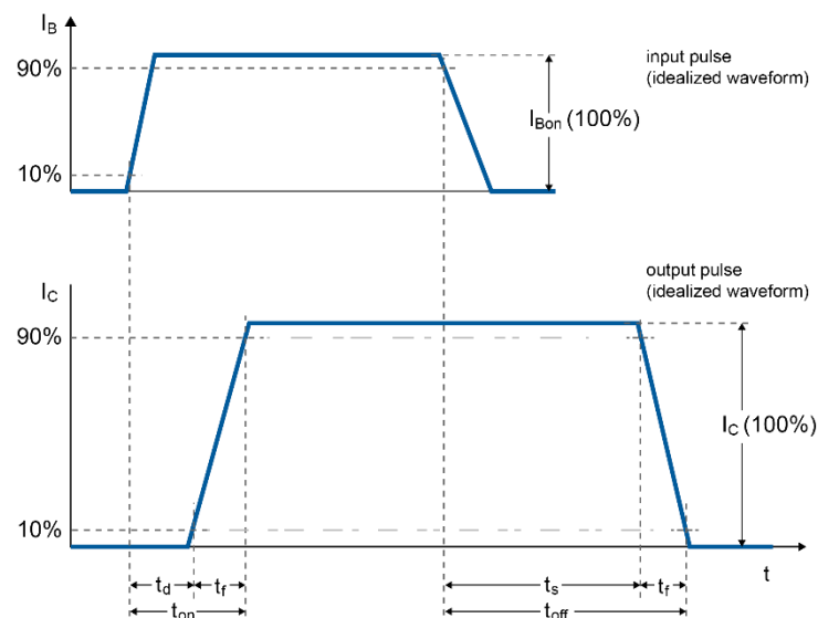
Fig 6. Timing Waveform
