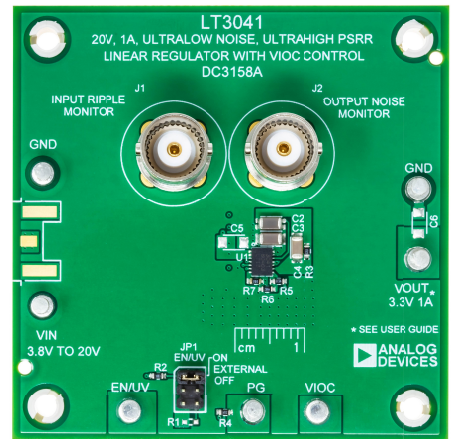
Figure 1. DC3158A Evaluation Board Photograph
