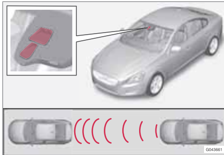
Location of the laser sensor in the windshield
