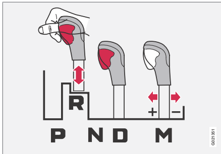
Shiftgate positions 1
