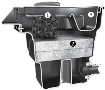
BioFalls Filter
