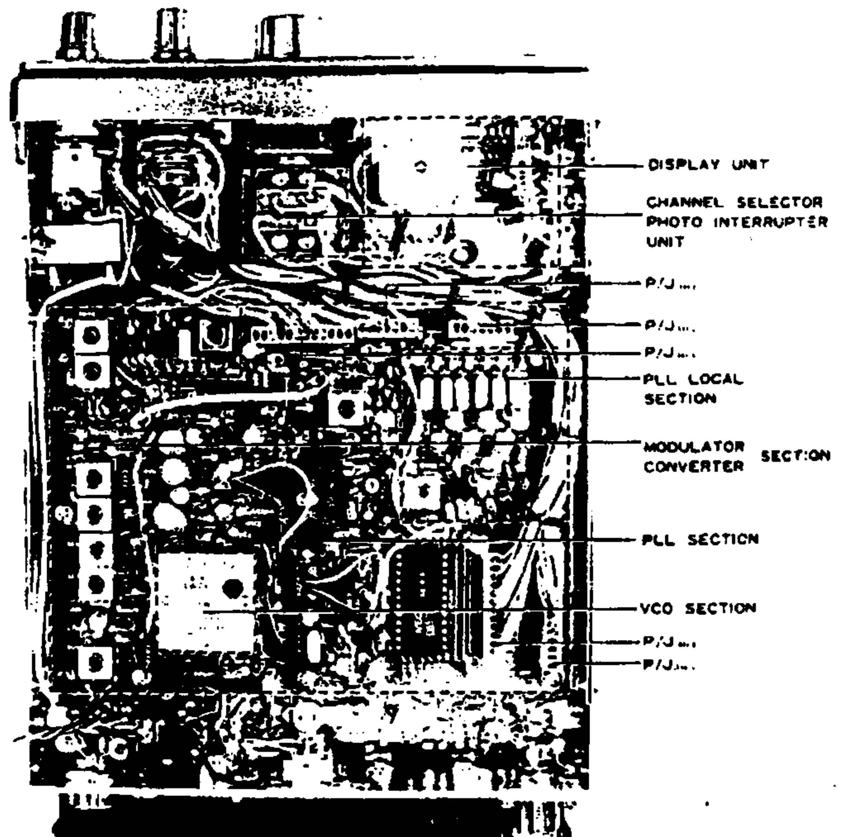
Figure 11 BOTTOM VIEW
