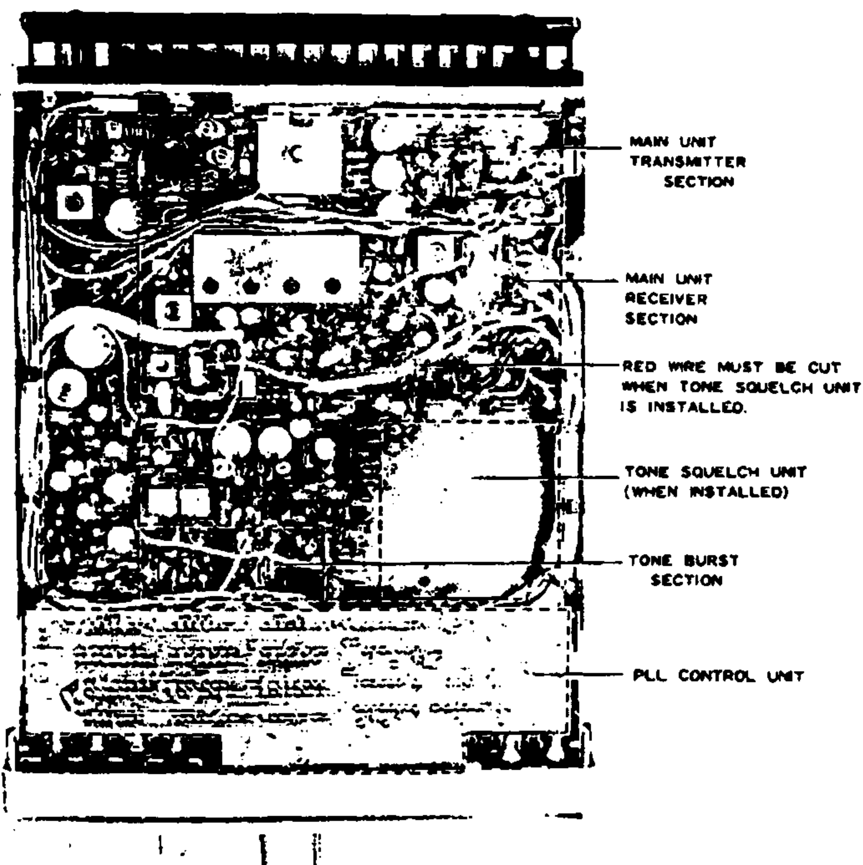
Figure 10 TOP VIEW
