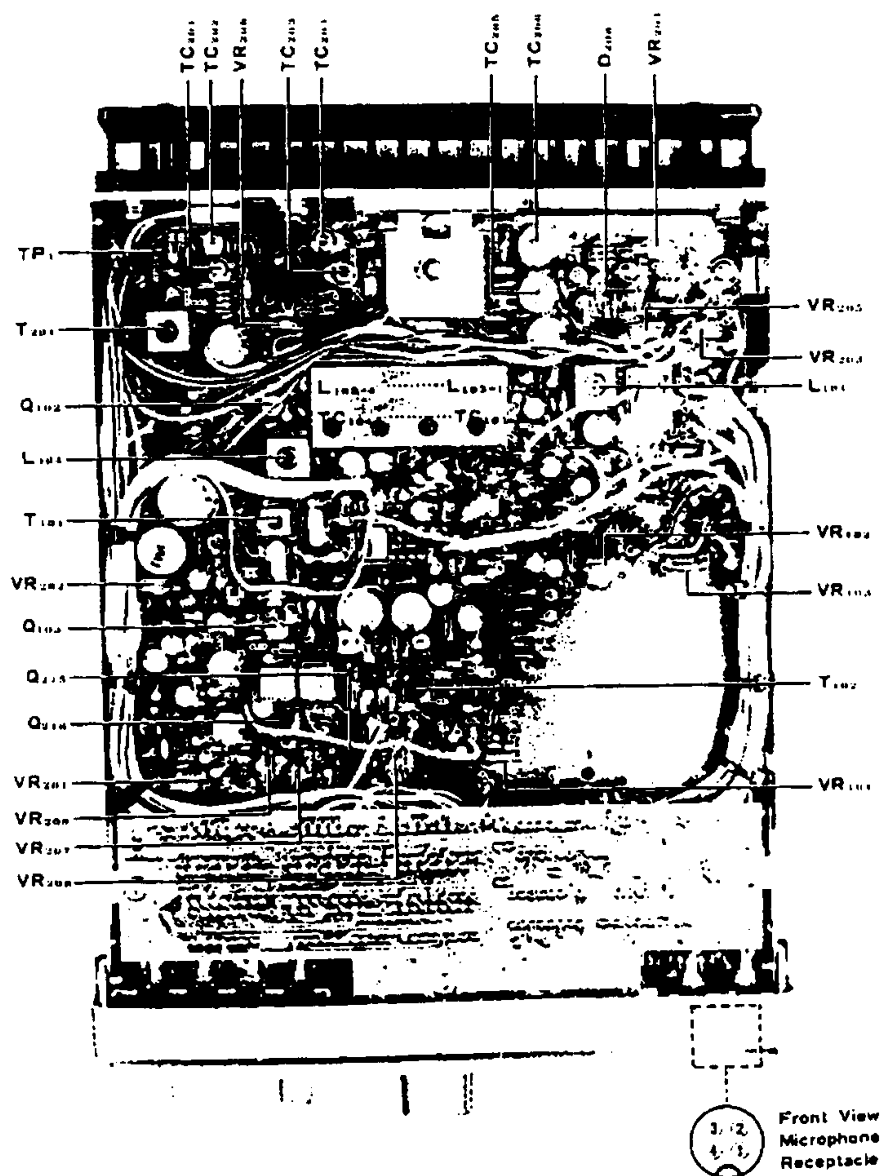
Figure 12 ALIGNMENT POINT
