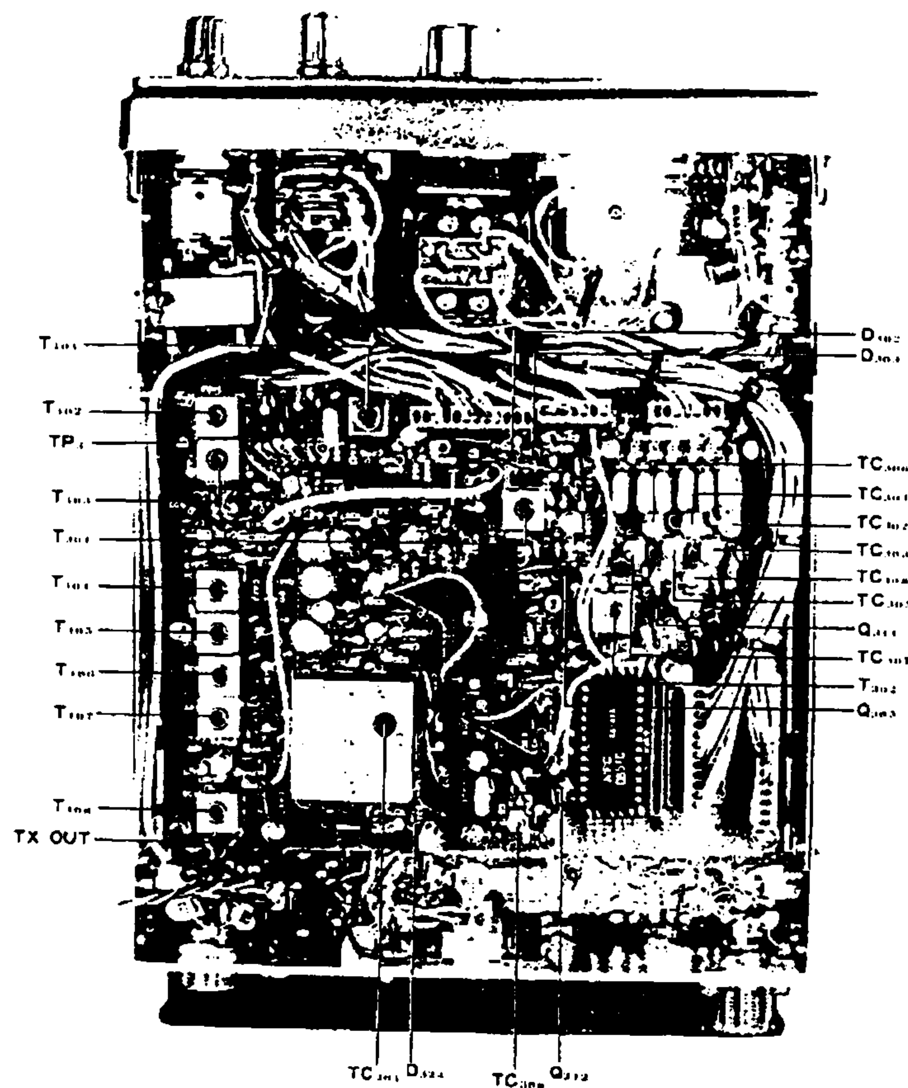
Figure 16 ALIGNMENT POINT
