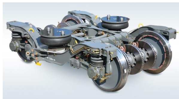
SF500 bogie
