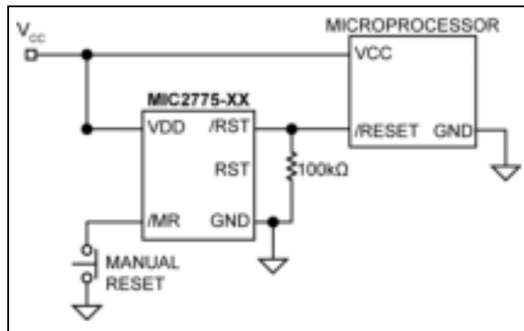
FIGURE 4-1: Valid \overline{\text{RST}} Below 1.2V.
