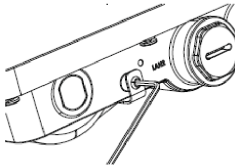
Figure 10: Securing the Mount Screw
