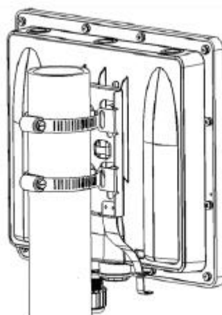
Figure 6: Mounting the Device
