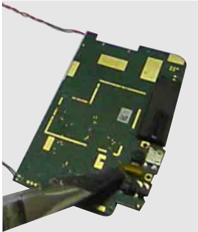
Figure 6. Removal steps of camera
