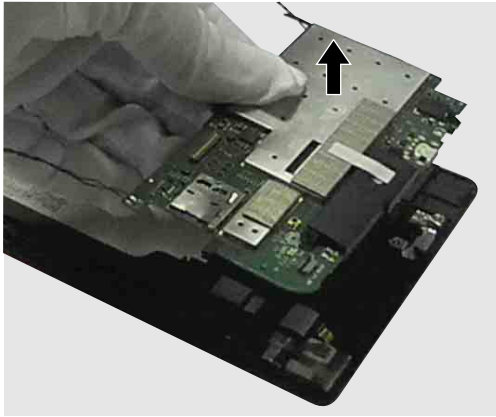
Figure 5. Removal steps of system board (continued)
