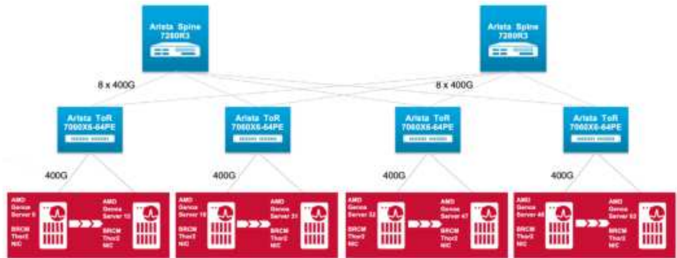
Figure 7: Roce Setup
