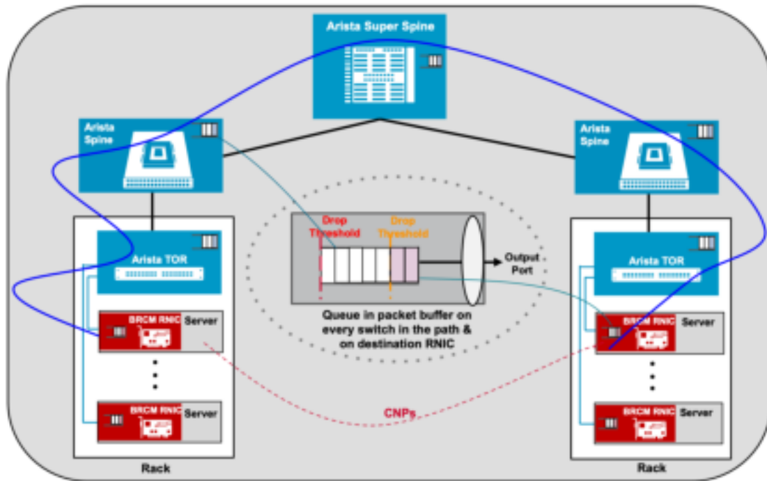
Figure 6: RoCE traffic in datacenter network
