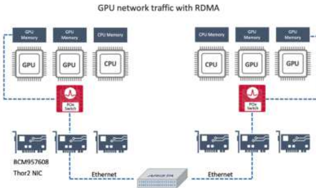
Figure 5: RoCE with Broadcom NICs and Arista Switch
