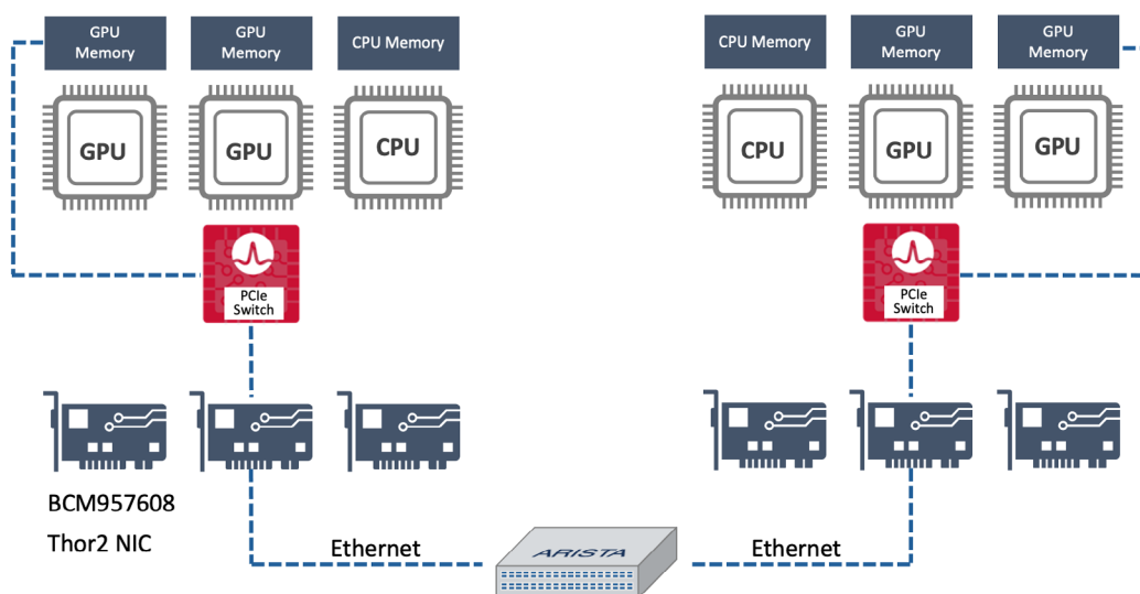
Figure 5: RoCE with Broadcom NICs and Arista Switch
