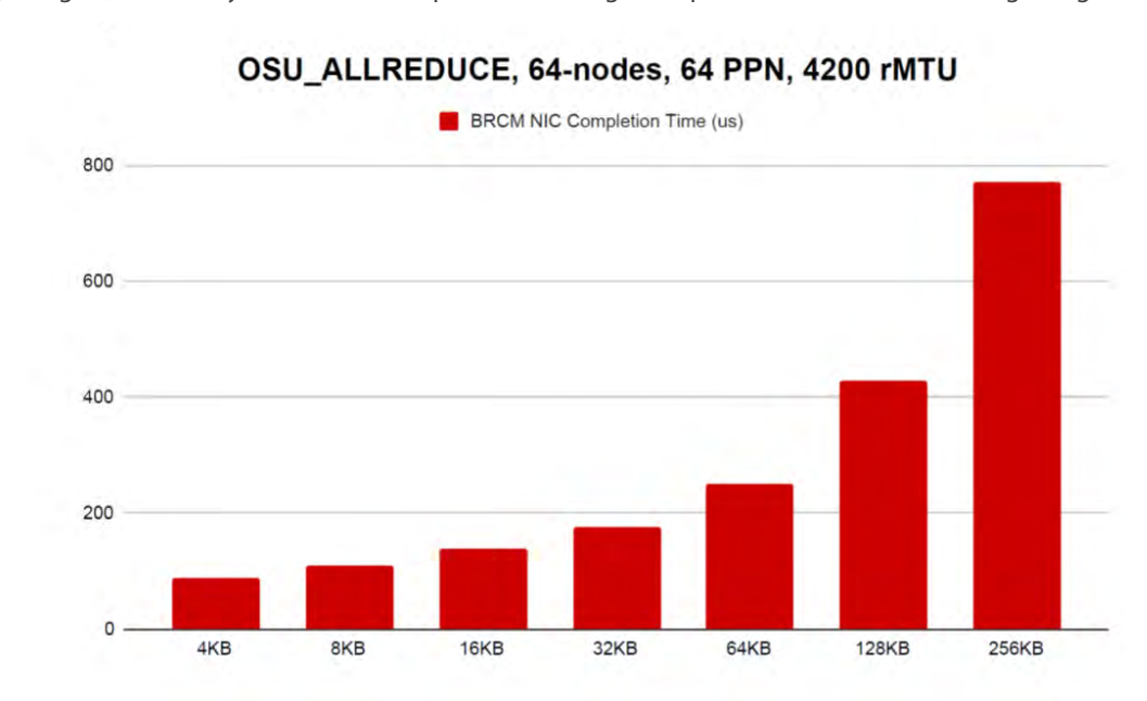
Figure 10: OSU All Reduce Latency Test with Broadcom NICs and Arista Switches on 400GE
