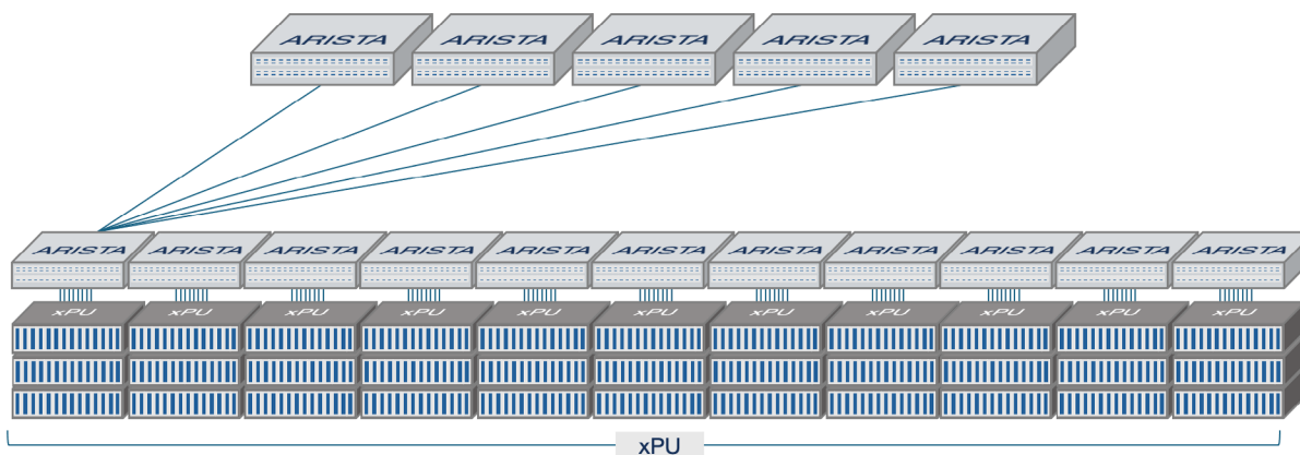
Figure 3: Leaf Spine Topology
