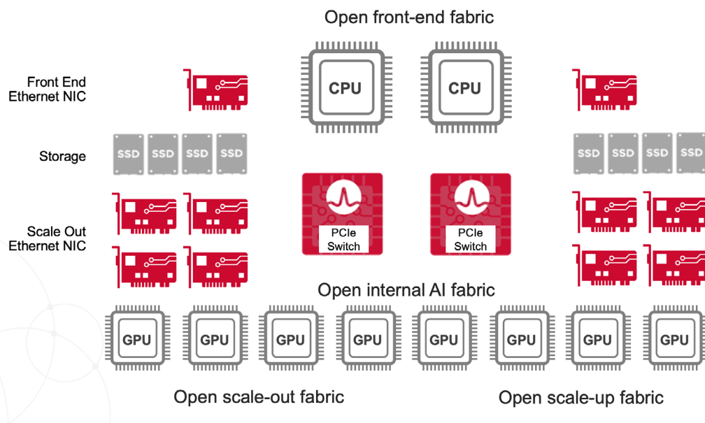
Figure 1: Basic AI server architecture
