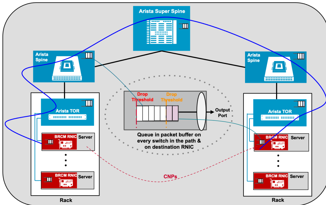
Figure 6: RoCE traffic in datacenter network
