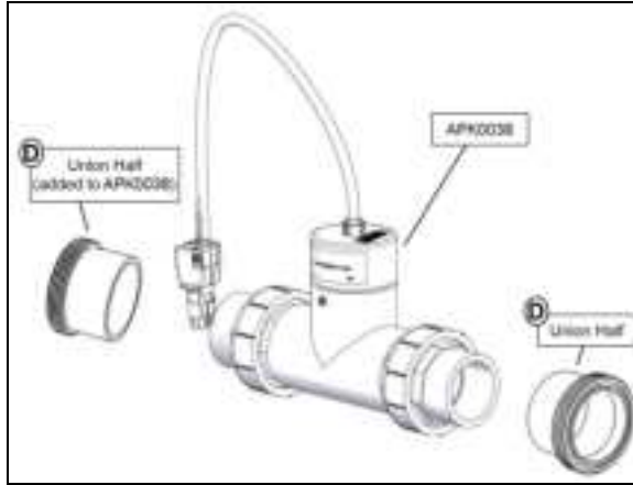
APK0065 (Inline Conversion Kit)
