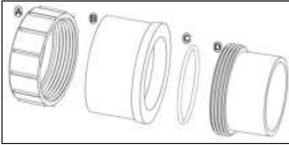
PLS2627 (Union Kit)
