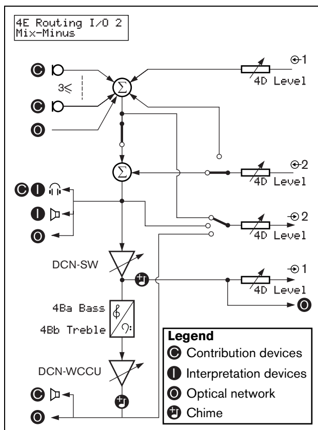
figure 12.4: Mix-minus
