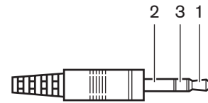
figure 14.14: 3.5 mm headphones plug, connection
