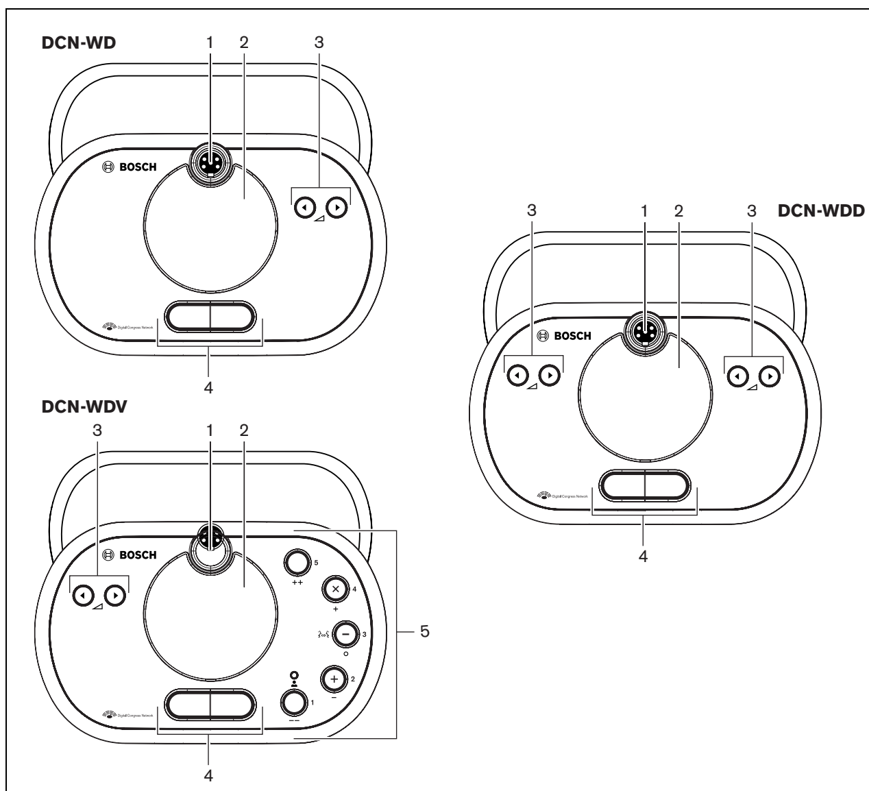
figure 14.1: Top views (1)
