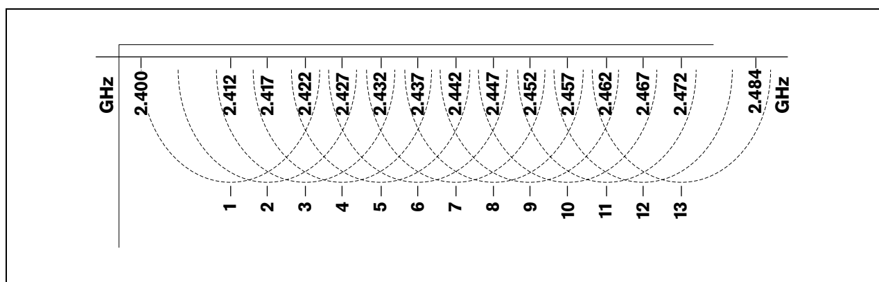
figure 1.1: WLAN channels
