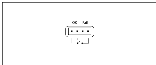
figure 10.10: Fault contact
