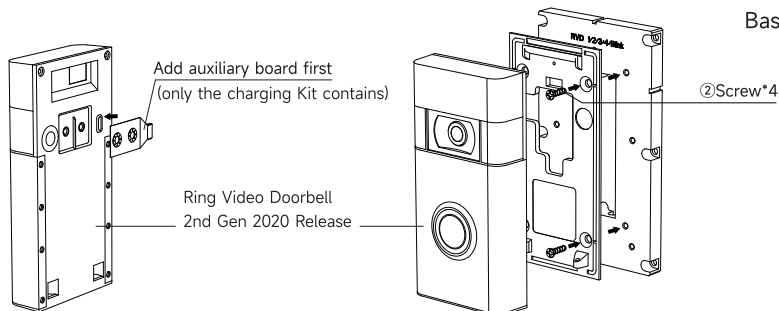
Base Plate
