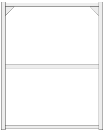
Wall frame with shelves H30" available in W18×D6" W24×D6" W18×D12" W24×D12"
