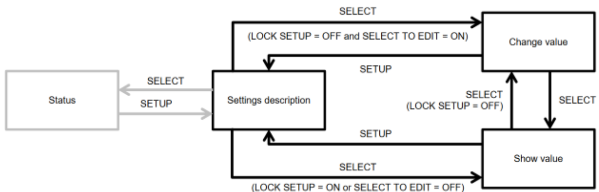
MPPT Control setting navigation chart
