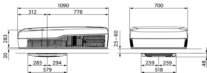
FreshJet FJX7457IHP
