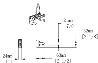
Hoisting Installation
