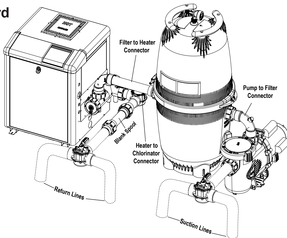
Figure 10. CV Standard Installation Diagram
