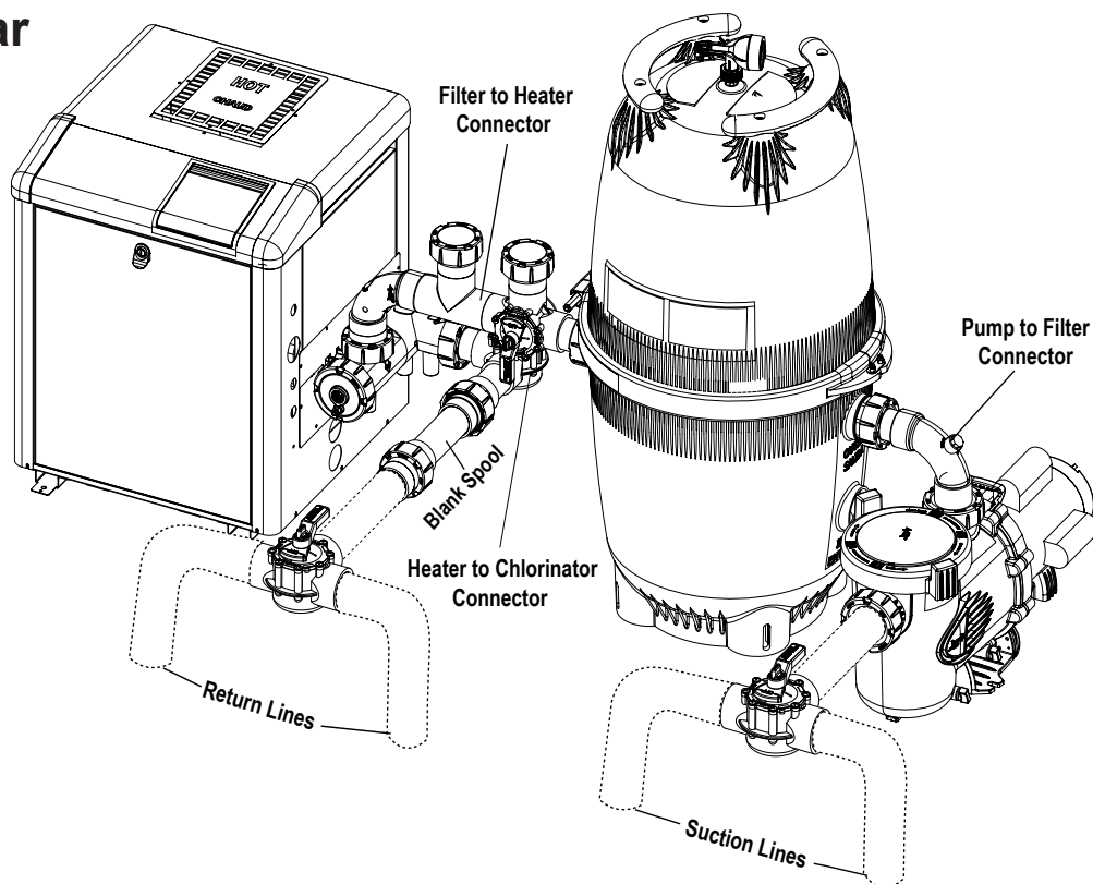
Figure 11. CV Solar Installation Diagram
