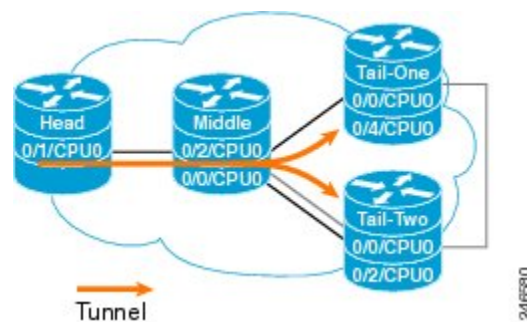
Figure 29: P2MP Topology
