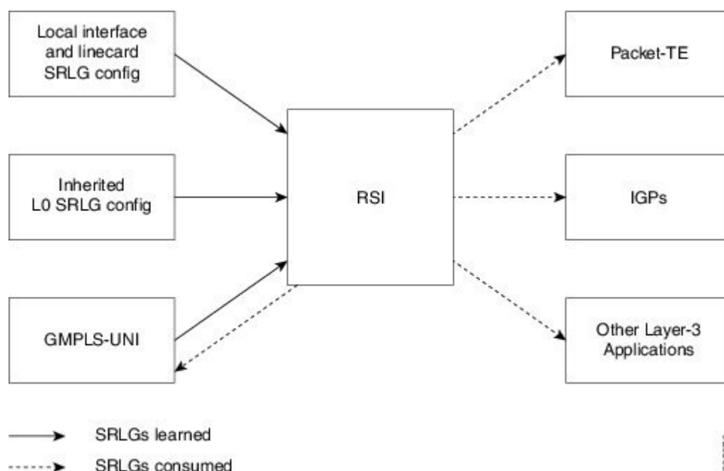
Figure 30: SRLG Communication
