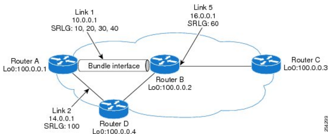
Figure 20: Shared Risk Link Group
