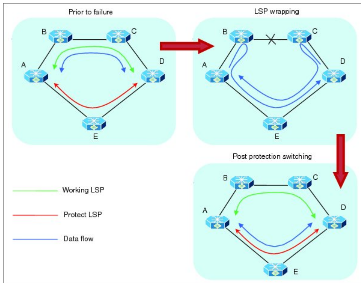
Figure 35: MPLS-TP LSP Wrapping Mechanism
