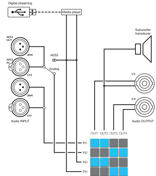
Default routing diagram.
