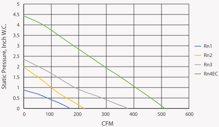
New Rn Fan Curves
