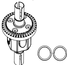
FTX10104 Complete differential
