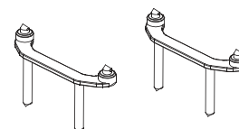
FTX10229 Body post 1set
