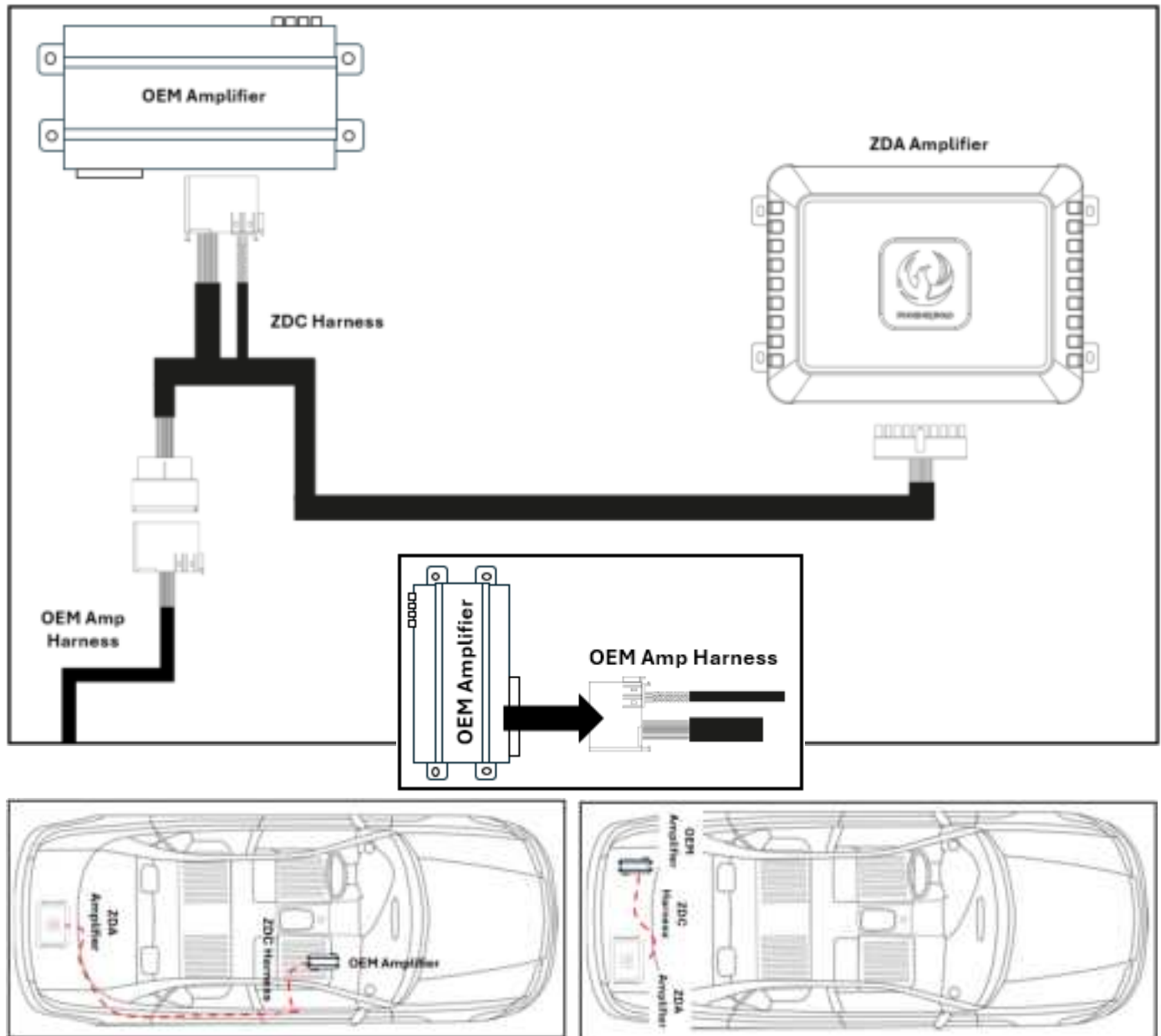
Example: OEM Amplifier located under front seat
