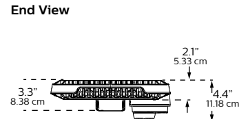
End View
