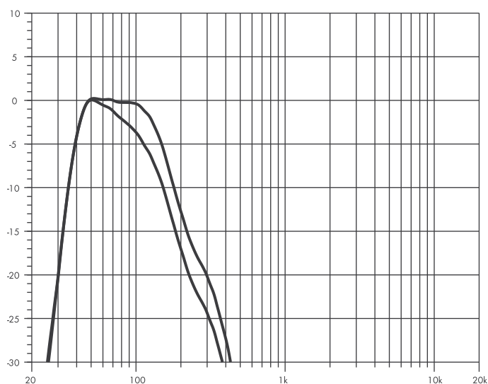
CCL-SUB frequency response, Standard and 100 modes
