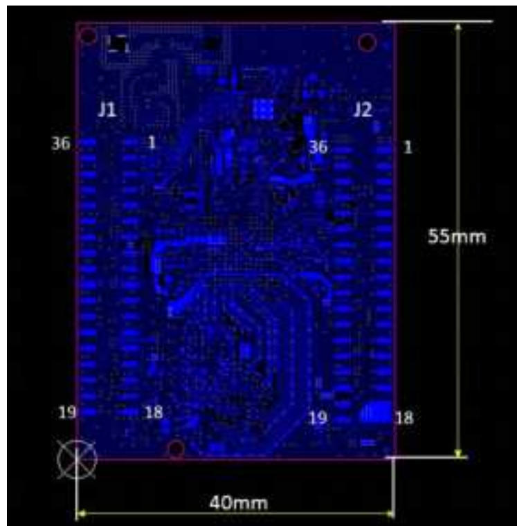
Figure 7.1-3: LS10 Top View - Mechanical Dimension 1
