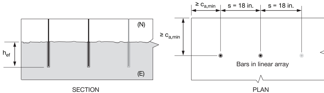
Illustration of Table 92 dimensions
