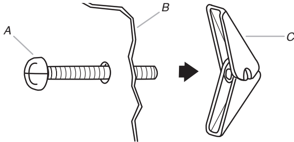
A. 3/16-24 x 3" round-head bolt B. Mounting plate C. Spring toggle nut
