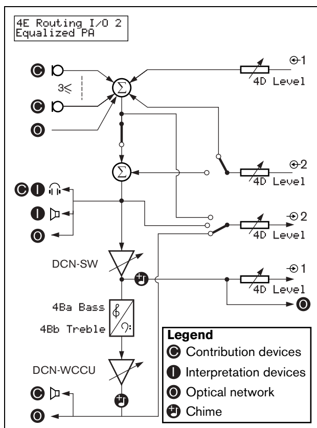
figure 12.2: Equalized PA
