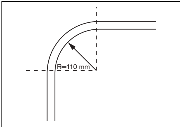
figure 3.3: Bend radius
