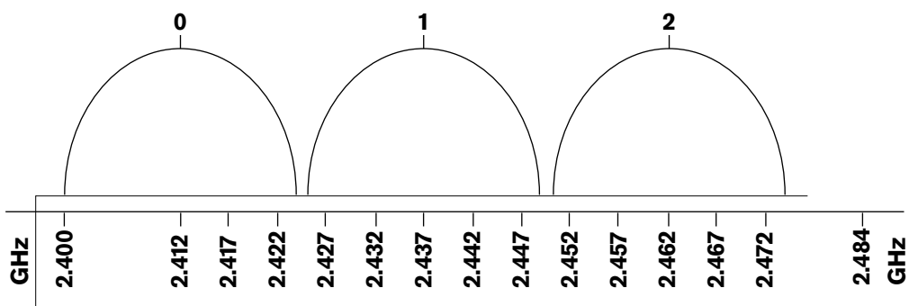
figure 1.2: DCN wireless carriers
