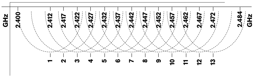
figure 1.1: WLAN channels
