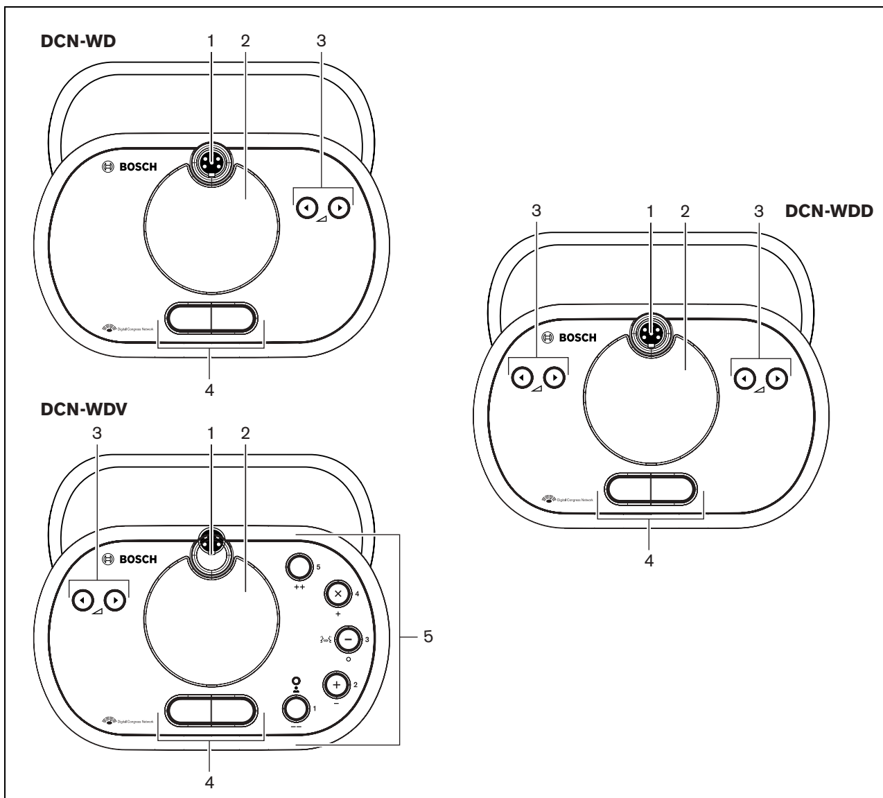
figure 14.1: Top views (1)
