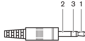
figure 14.14: 3.5 mm headphones plug, connection
