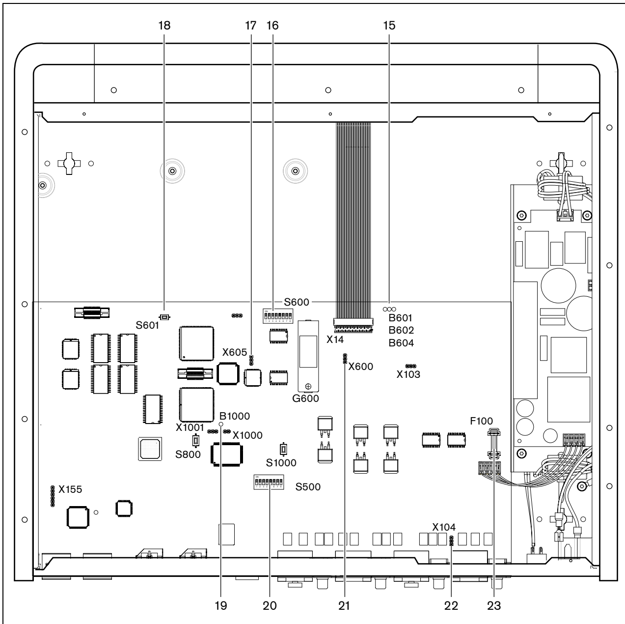
figure 10.2: Internal settings
