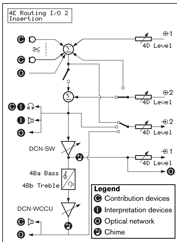
figure 12.3: Insertion
