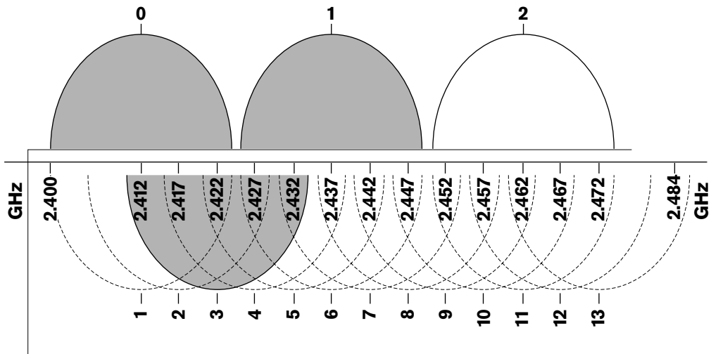
figure 1.3: Example of interference
