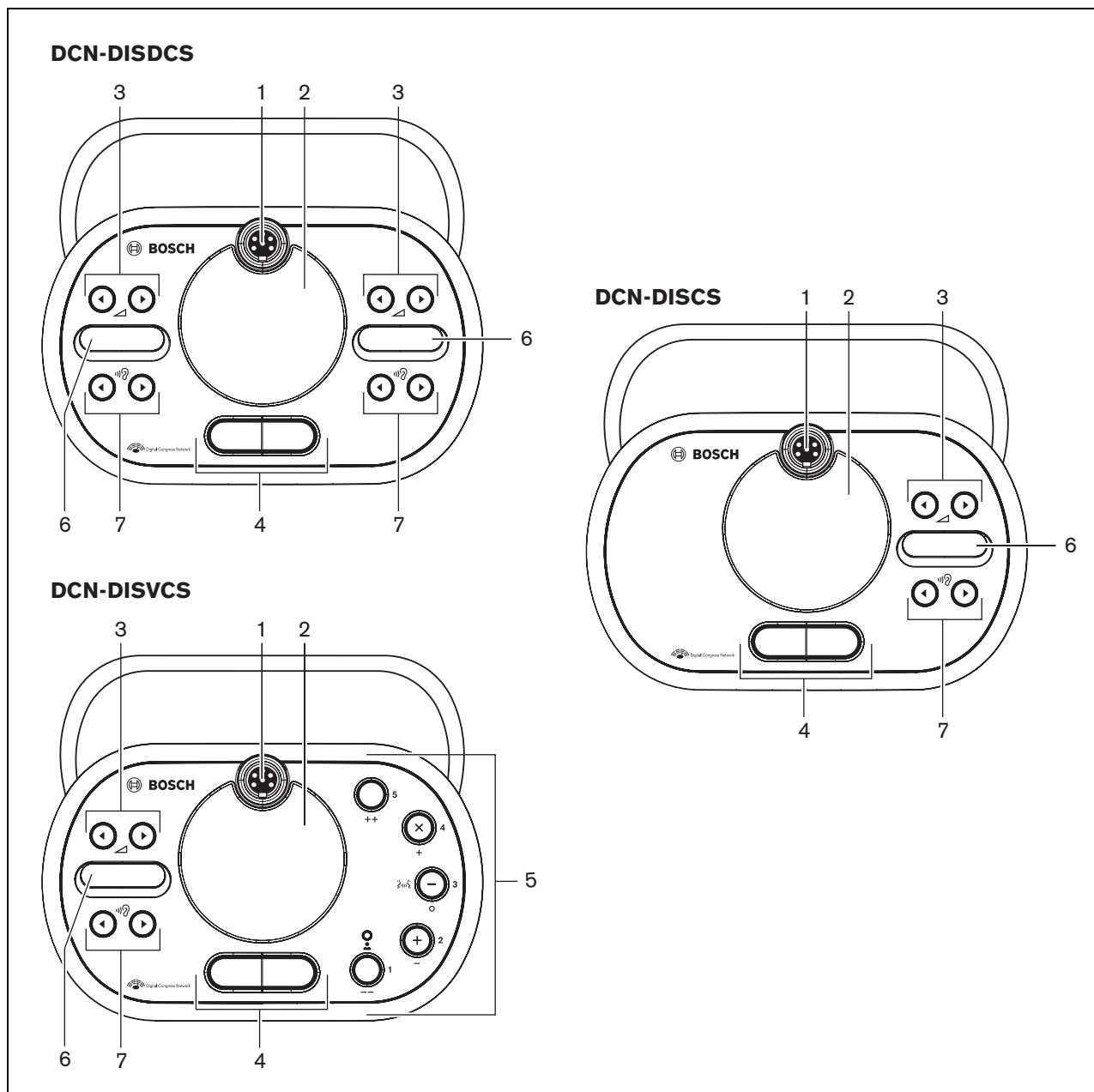
figure 14.2: Top views (2)
