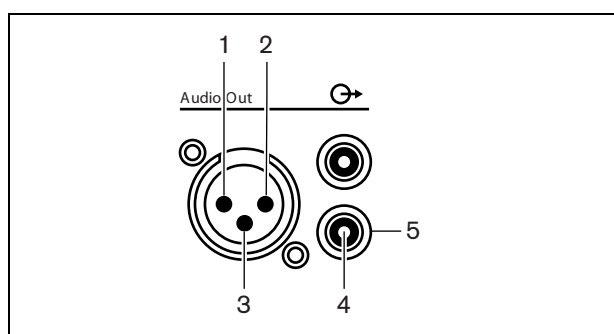
figure 10.9: Audio output, connection
