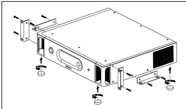
figure 10.3: Installation
