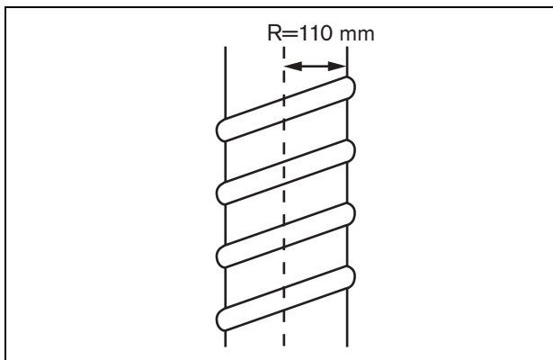
figure 3.4: Coiling radius
