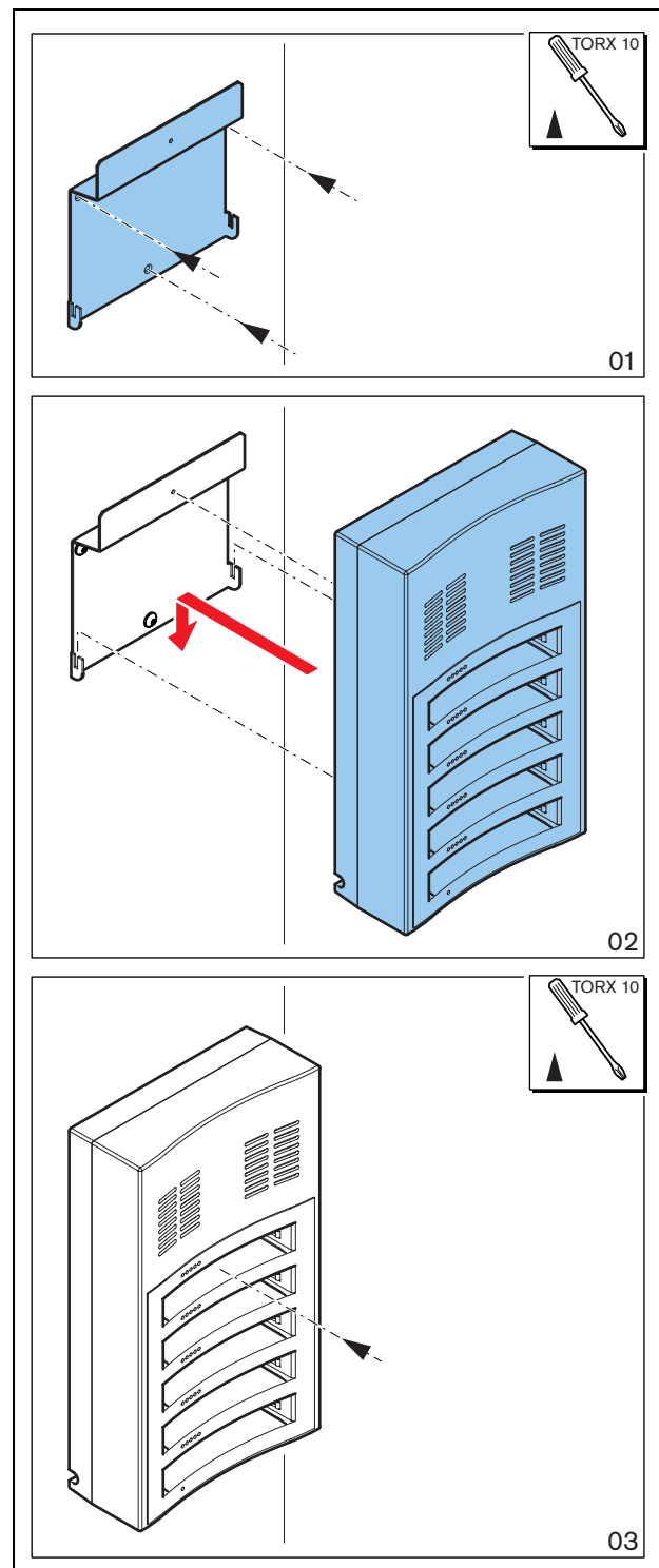
figure 17.2: Installation, wall
