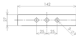
Bracket Dimensions
