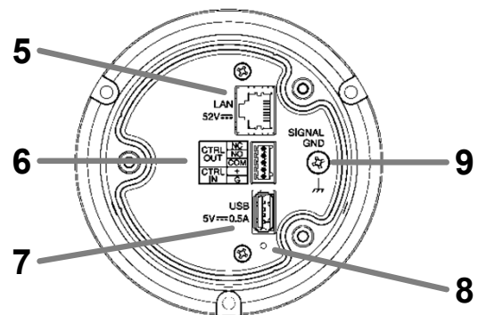
Rear Panel without Back Cover
