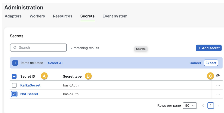
Figure 14: Secrets table
