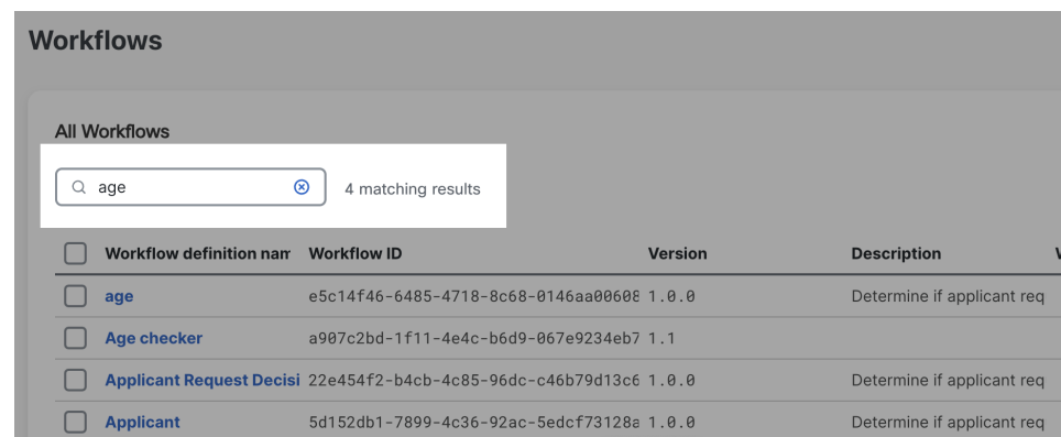
Figure 4: Filter option
