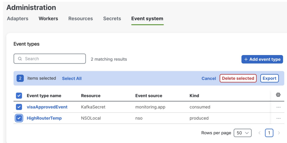
Figure 15: Event system
