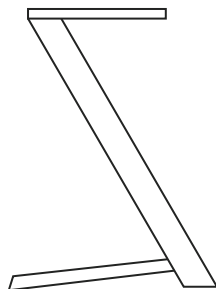
1 Table leg Qty 2 (20.86x0.98x28.11")
