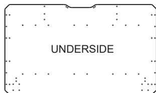
5 Table top Qty 1 (39.37x23.62x0.59")
