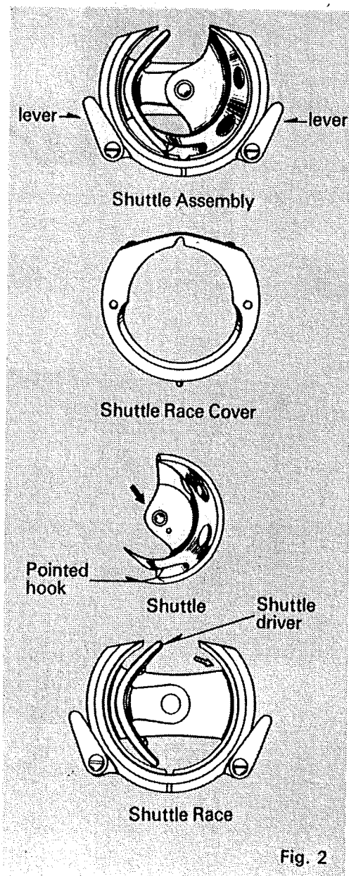
Fig. 2 Parts of the Shuttle Assembly
