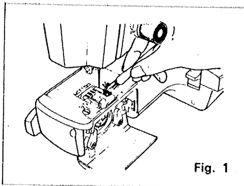
Fig. 1 Cleaning the feed dogs with a brush.
