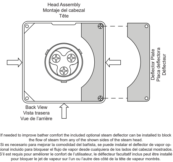
Figure 12 - Optional Deflector
