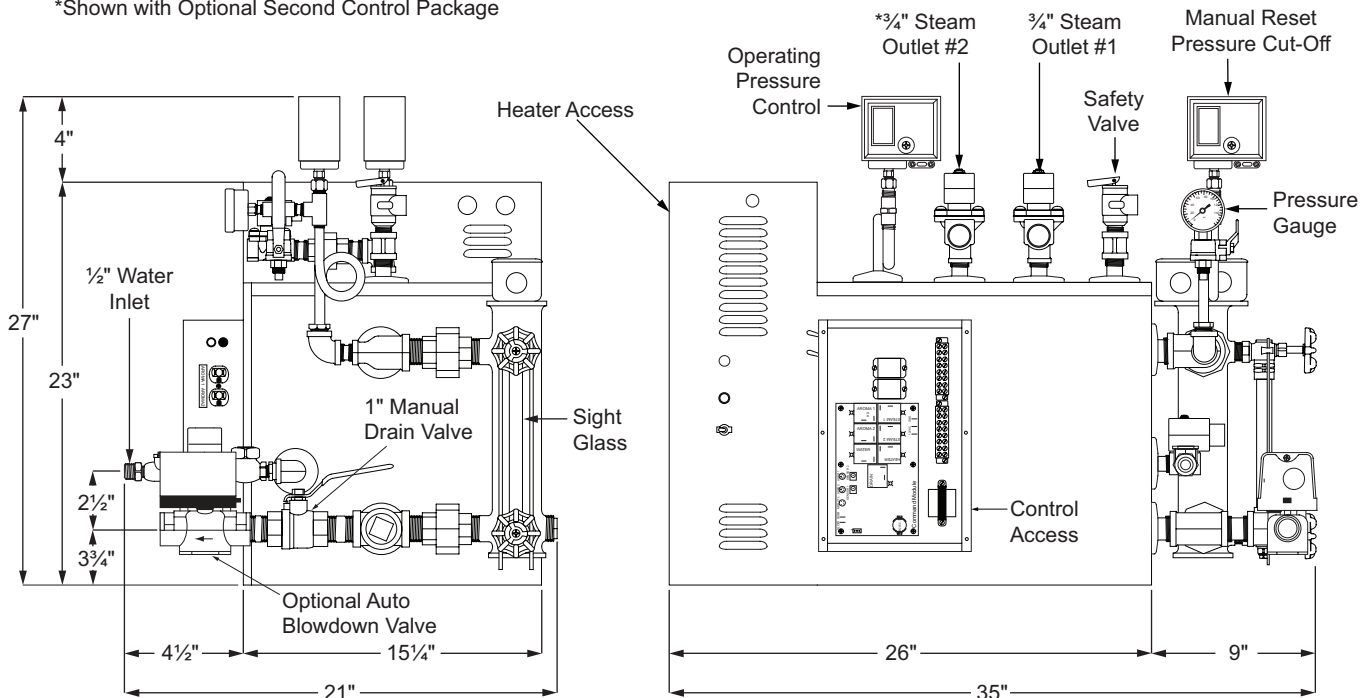
Figure 2 - Dimensional Drawing for Heavy Commercial Steam Generator
