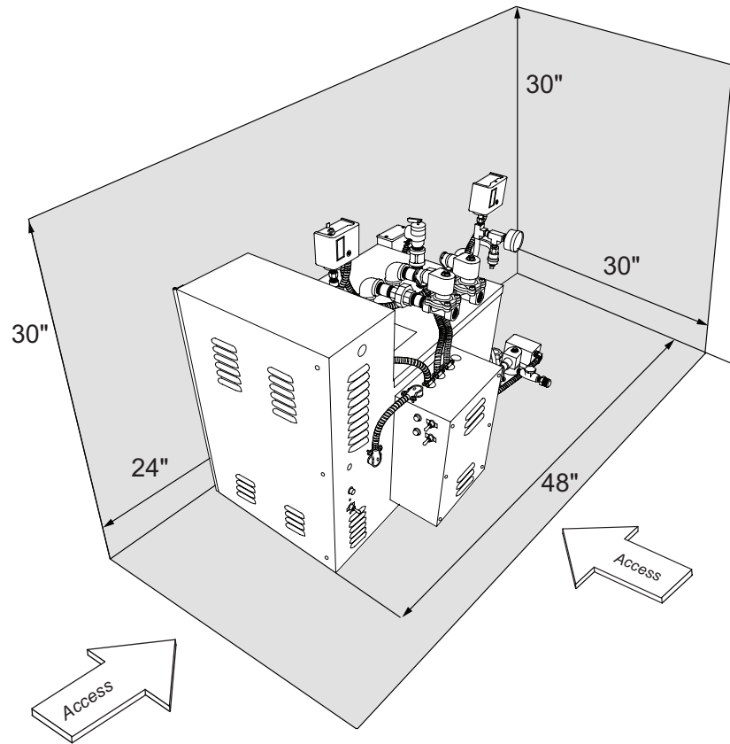
Figure 1 - Access Requirements
