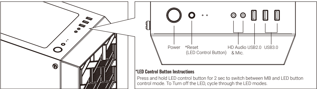
I/O Panel
