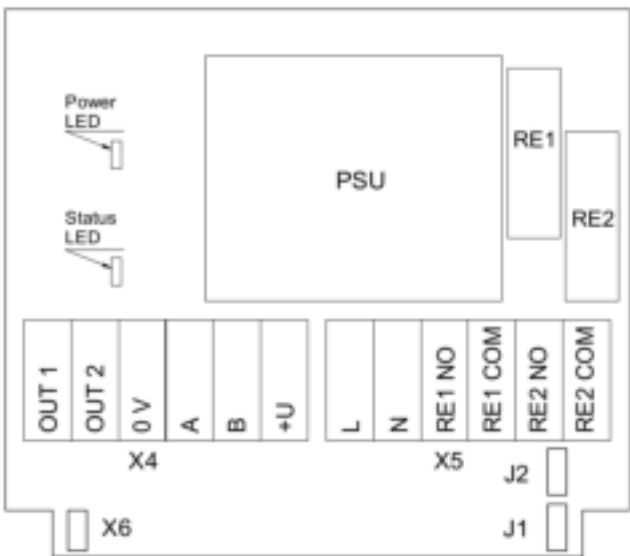
Version with PSU
