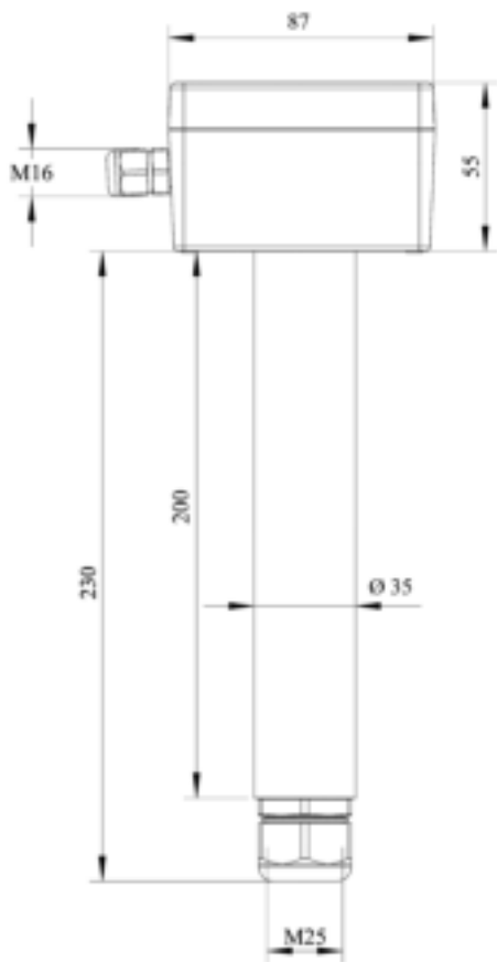
Duct mount version
