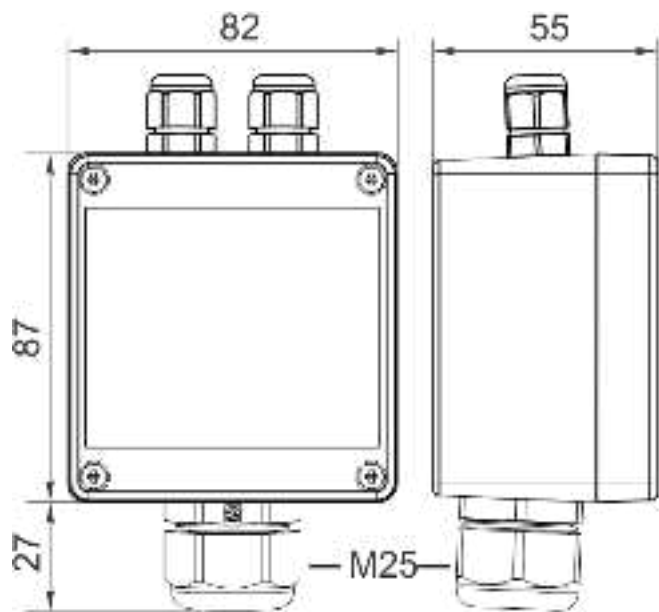
Wall mount version
