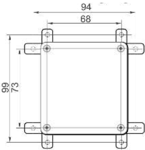
with mounting lugs
